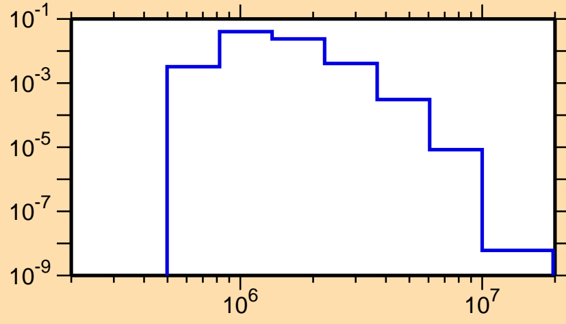
\sigma vs. E for ^{157}\text{Lu}(n,n_4)
