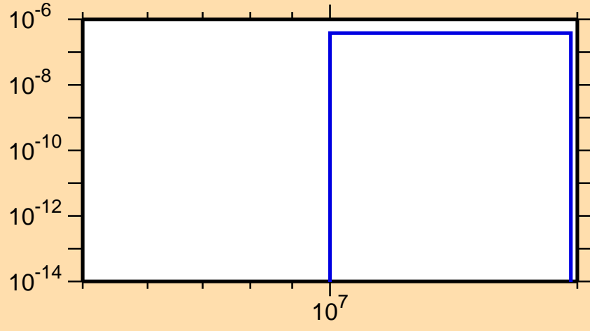
\sigma vs. E for ^{157}\text{Lu}(n,nd)
