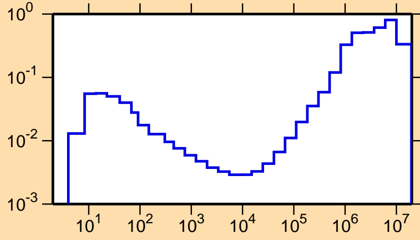
\sigma vs. E for ^{157}\text{Lu}(n,\text{inel.})
