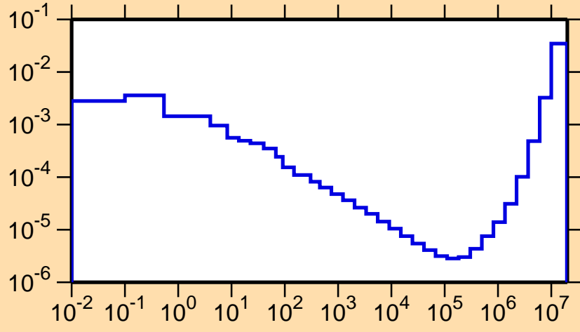
\sigma vs. E for ^{157}\text{Lu}(n,p\alpha)
