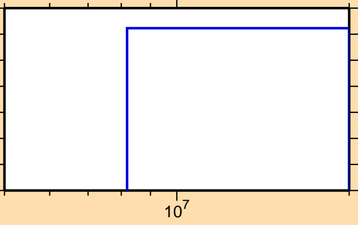
\sigma vs. E for ^{157}\text{Lu}(n,\text{nd})
