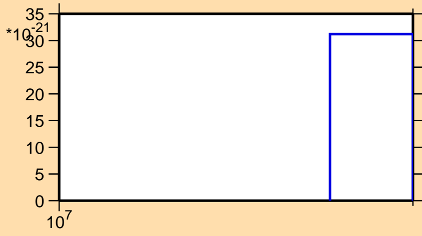
\sigma vs. E for ^{158}\text{Lu}(\text{mt } 11)
