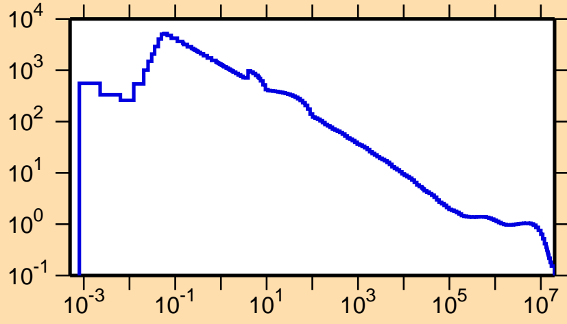
\sigma vs. E for ^{158}\text{Lu}(n,p)
