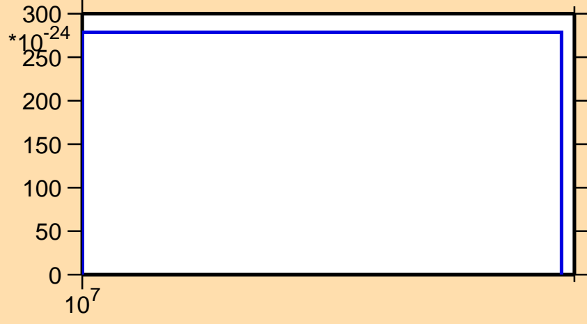
\sigma vs. E for ^{158}\text{Lu} (mt 11)
