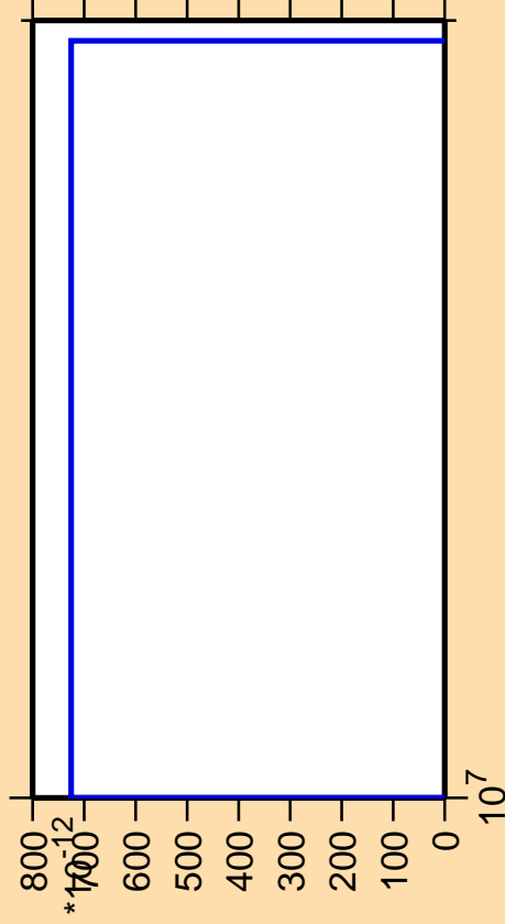
\Delta\sigma/\sigma vs. E for ^{158}\text{Lu} (mt 11)
