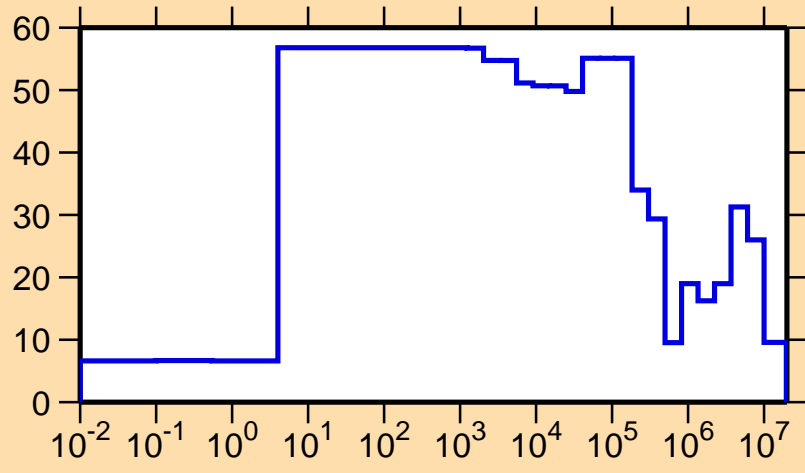
\Delta\sigma/\sigma vs. E for ^{158}\text{Lu}(n,\text{el.})
