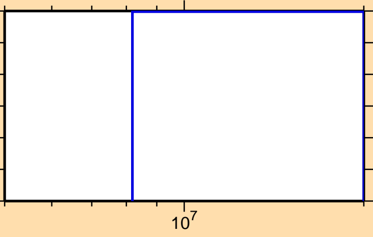
\sigma vs. E for ^{158}\text{Lu}(n,\text{pt})
