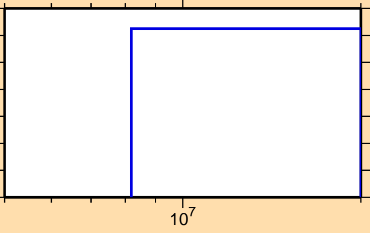
\sigma vs. E for ^{158}\text{Lu}(n,\text{nd})
