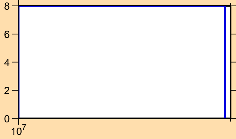
\Delta\sigma/\sigma vs. E for ^{159}\text{Lu}(n,\text{nonel.})
