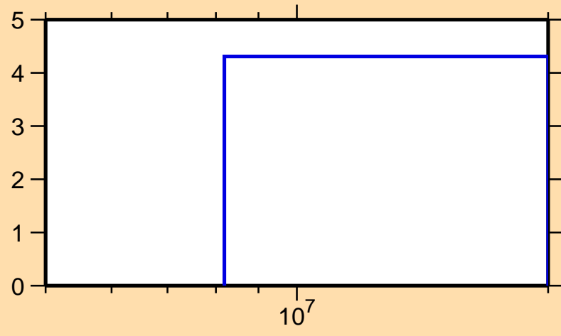
\Delta\sigma/\sigma vs. E for ^{159}\text{Lu}(n,\text{tot.})
