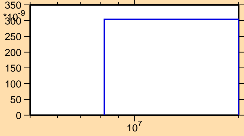
\sigma vs. E for ^{159}\text{Lu}(n,\text{pd})
