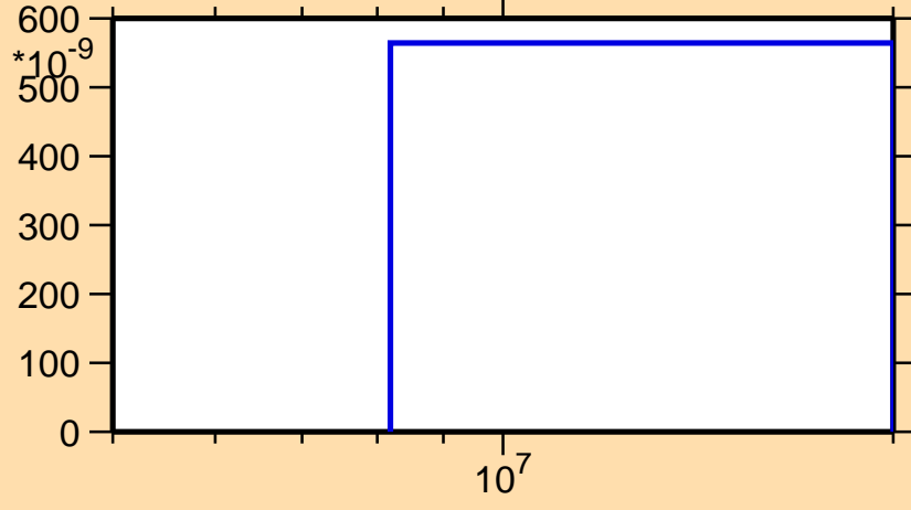
\sigma vs. E for ^{159}\text{Lu}(n,2n\alpha)
