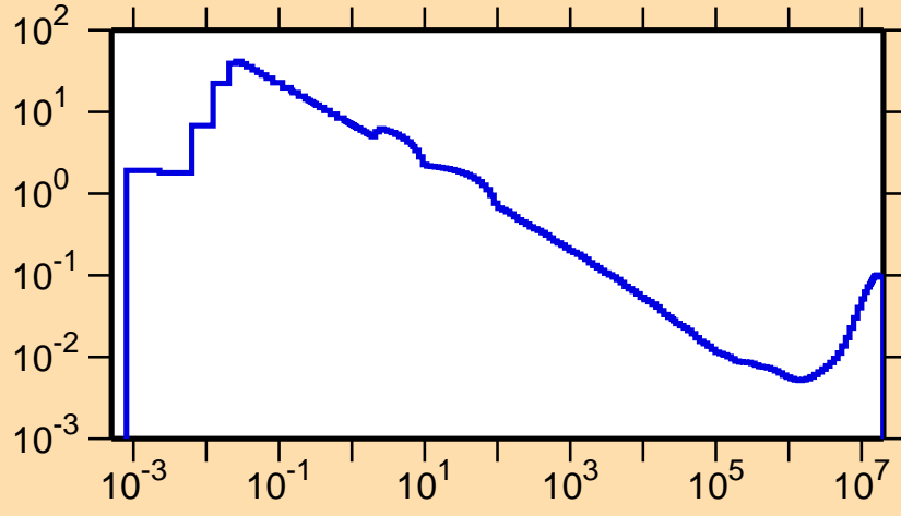
\sigma vs. E for ^{160}\text{Lu}(n,\alpha)
