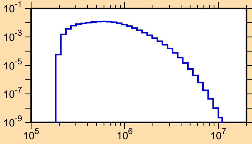
\sigma vs. E for ^{160}\text{Lu}(n,n_1)
