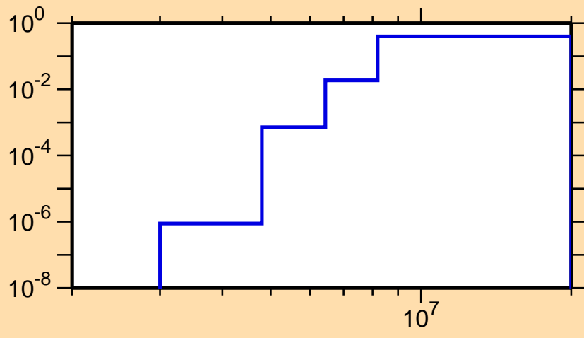
\sigma vs. E for ^{160}\text{Lu}(n,np)
