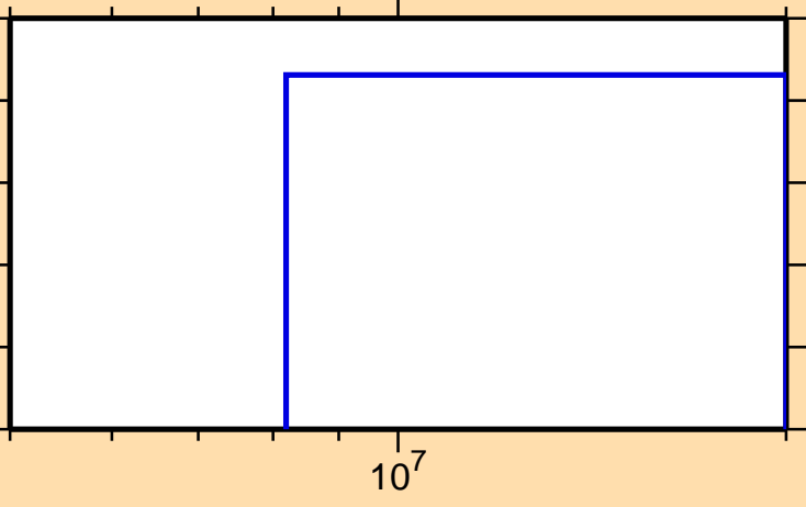
\sigma vs. E for ^{160}\text{Lu}(n,\text{nd})
