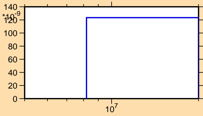
\sigma vs. E for ^{160}\text{Lu}(n,pd)
