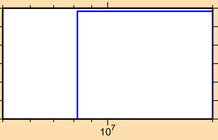
\sigma vs. E for ^{160}\text{Lu}(n,nt)
