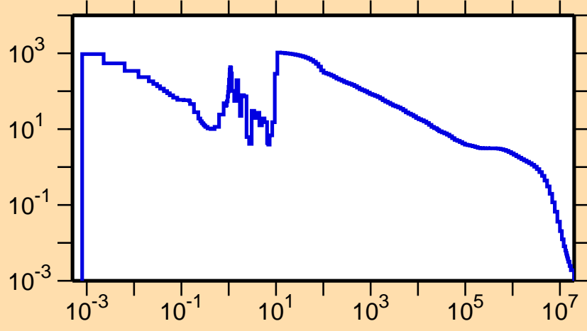
\sigma vs. E for ^{161}\text{Lu}(n,\gamma)
