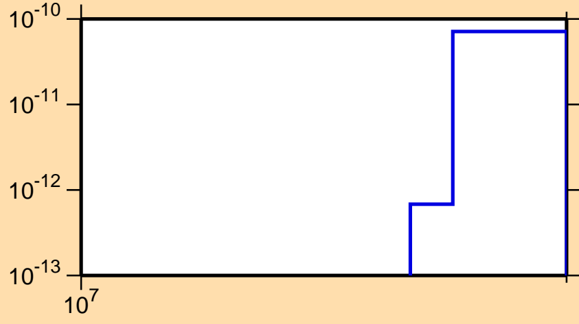
\sigma vs. E for ^{161}\text{Lu} (mt 34)
