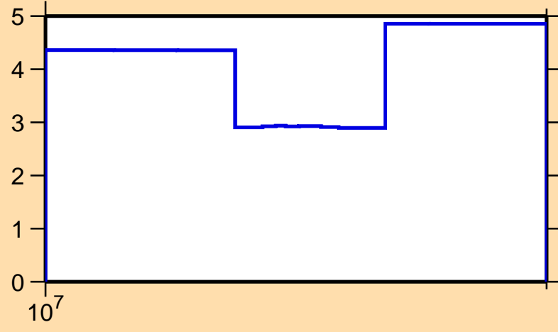
\Delta\sigma/\sigma vs. E for ^{161}\text{Lu}(n,\text{tot.})
