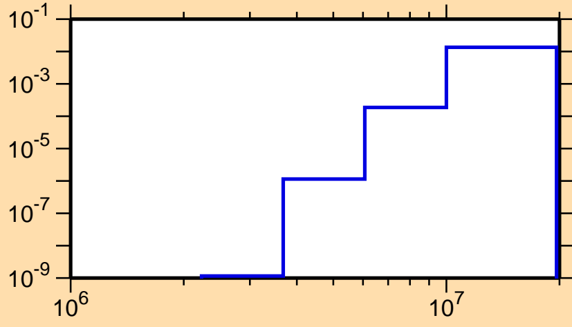
\sigma vs. E for ^{161}\text{Lu}(n,n\alpha)
