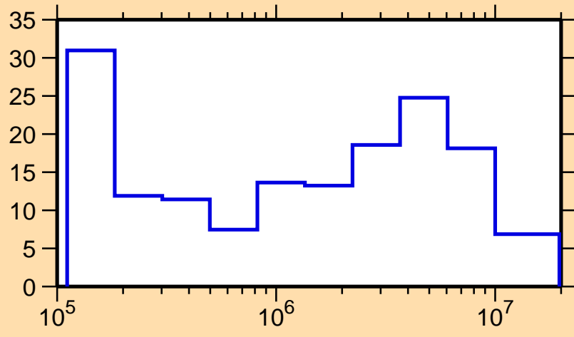
\Delta\sigma/\sigma vs. E for ^{161}\text{Lu}(n, el.)
