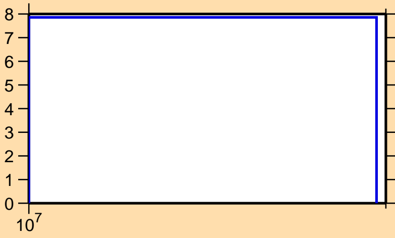
\Delta\sigma/\sigma vs. E for ^{161}\text{Lu}(n,\text{nonel.})
