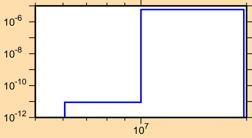
\sigma vs. E for ^{161}\text{Lu}(\text{mt } 45)
