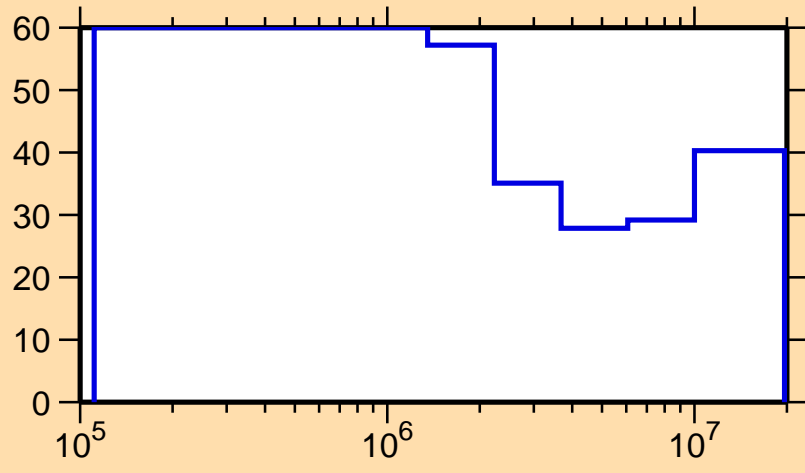
\Delta\sigma/\sigma vs. E for ^{161}\text{Lu}(n,n\text{cont.})
