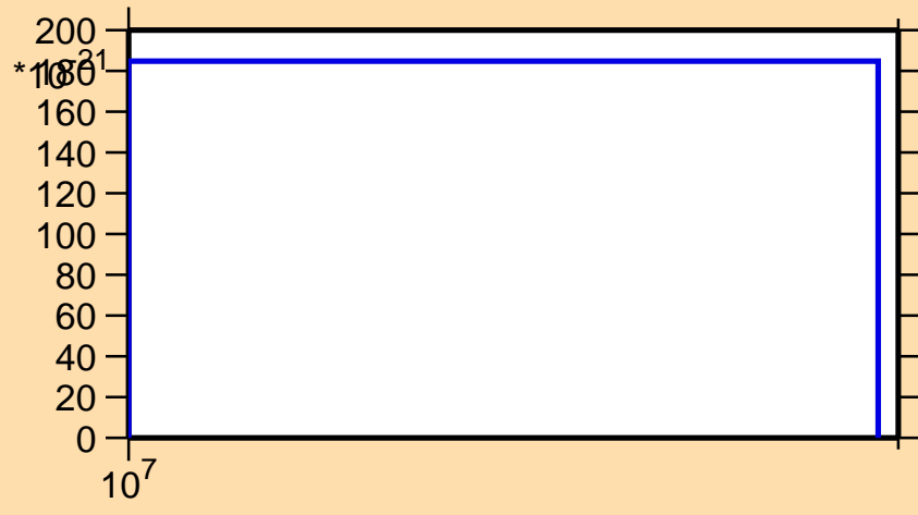
\sigma vs. E for ^{162}\text{Lu} (mt 11)
