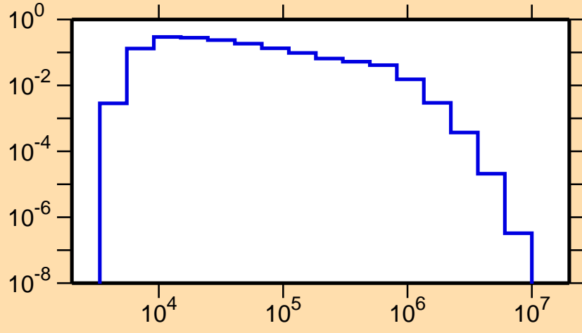
\sigma vs. E for ^{162}\text{Lu}(n,n_1)
