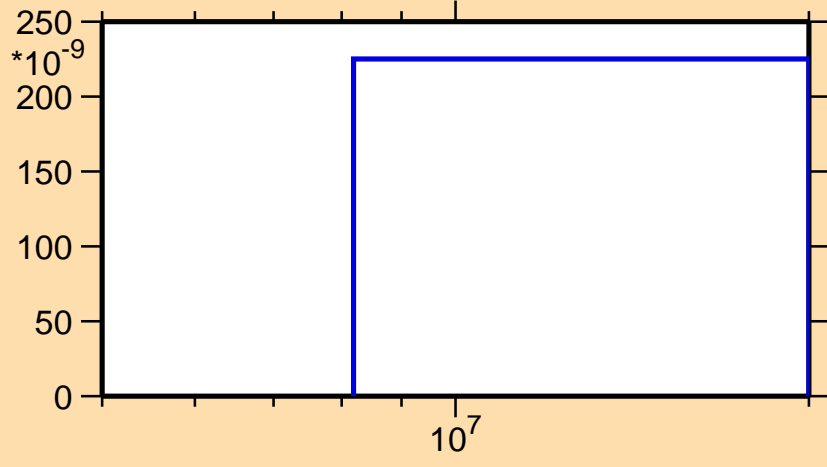
\sigma vs. E for ^{162}\text{Lu}(\text{mt } 45)
