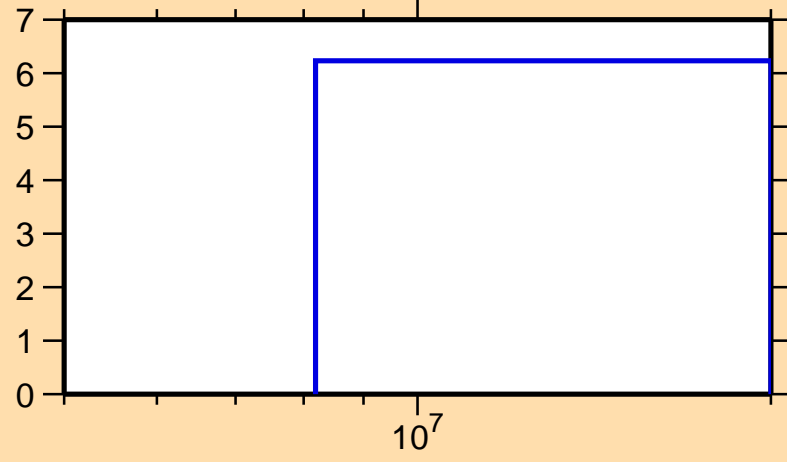
\Delta\sigma/\sigma vs. E for ^{162}\text{Lu}(n,\text{el.})
