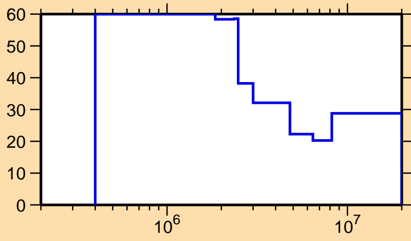
\Delta\sigma/\sigma vs. E for ^{162}\text{Lu}(n,n\text{cont.})
