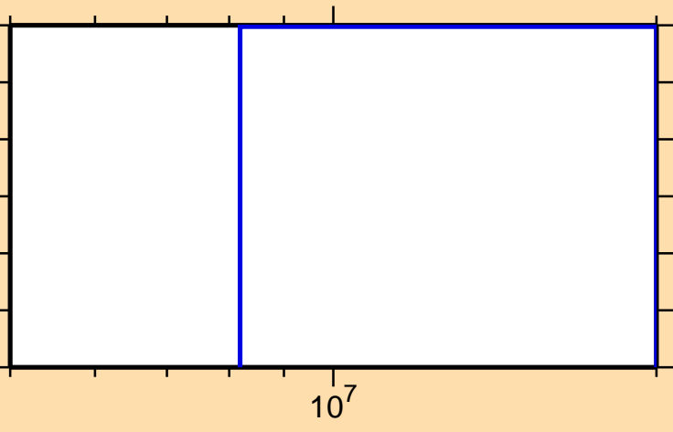
\sigma vs. E for ^{162}\text{Lu}(n,\text{pt})
