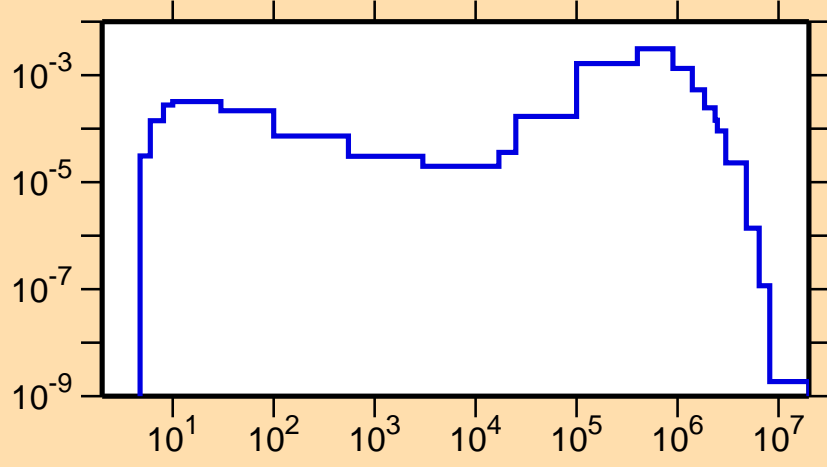
\sigma vs. E for ^{162}\text{Lu}(n,n_2)
