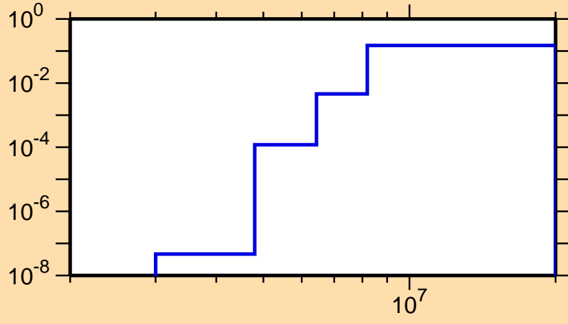
\sigma vs. E for ^{162}\text{Lu}(n,np)
