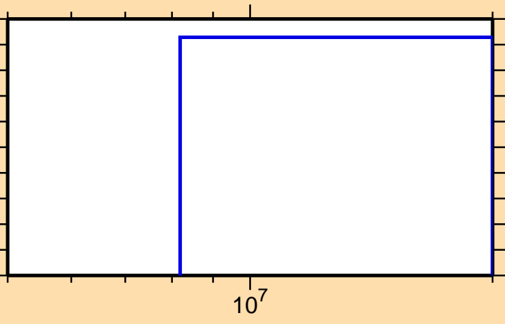
\sigma vs. E for ^{162}\text{Lu}(\text{mt117})
