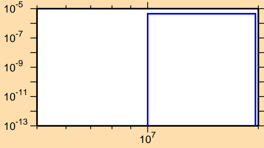
\sigma vs. E for ^{162}\text{Lu}(n,nd)
