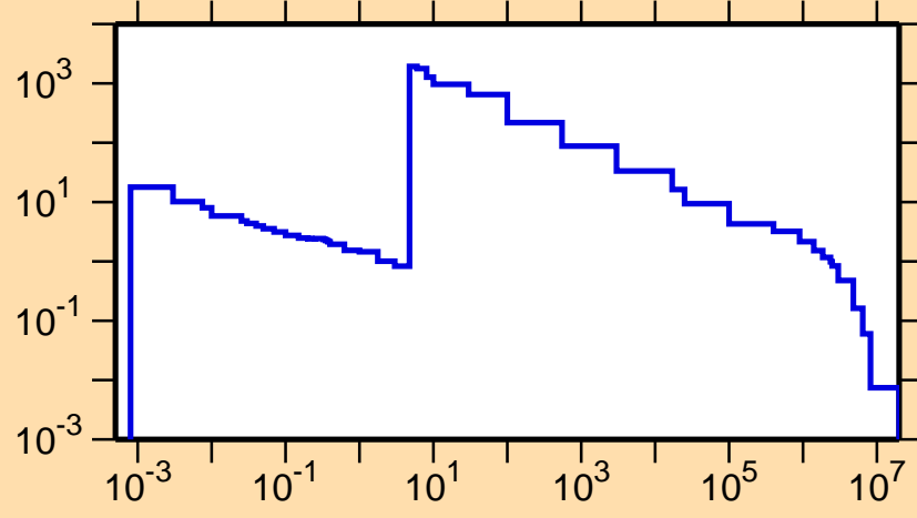
\sigma vs. E for ^{162}\text{Lu}(n,\gamma)
