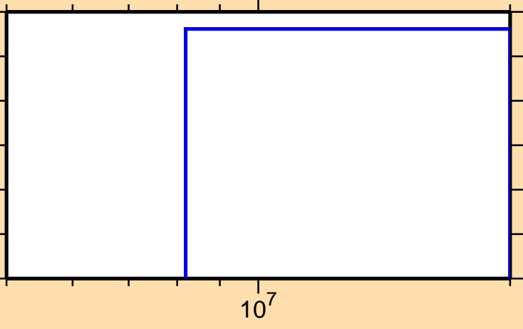
\sigma vs. E for ^{162}\text{Lu}(n,2n\alpha)
