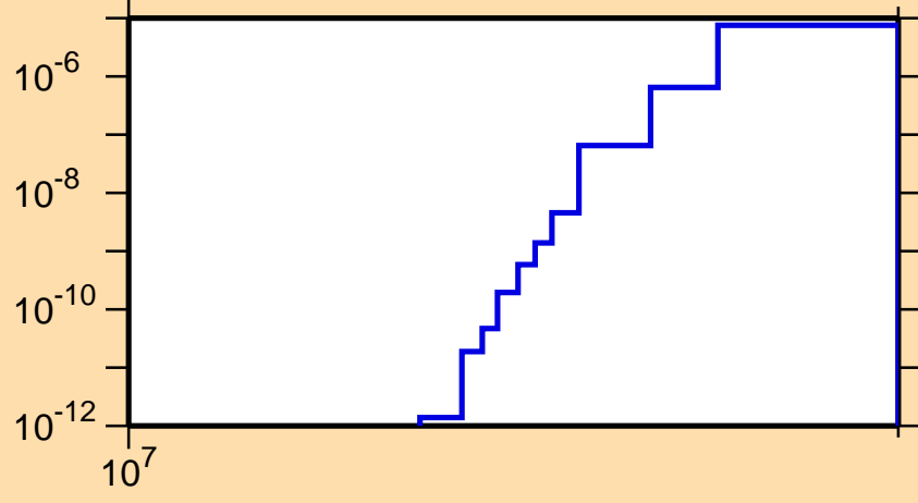
\sigma vs. E for ^{163}\text{Lu}(n,\text{nd})
