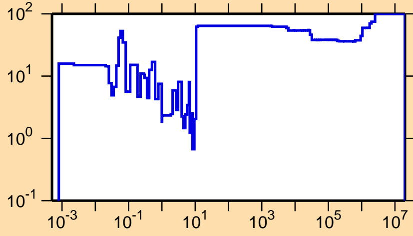
\Delta\sigma/\sigma vs. E for ^{163}\text{Lu}(n,\gamma)
