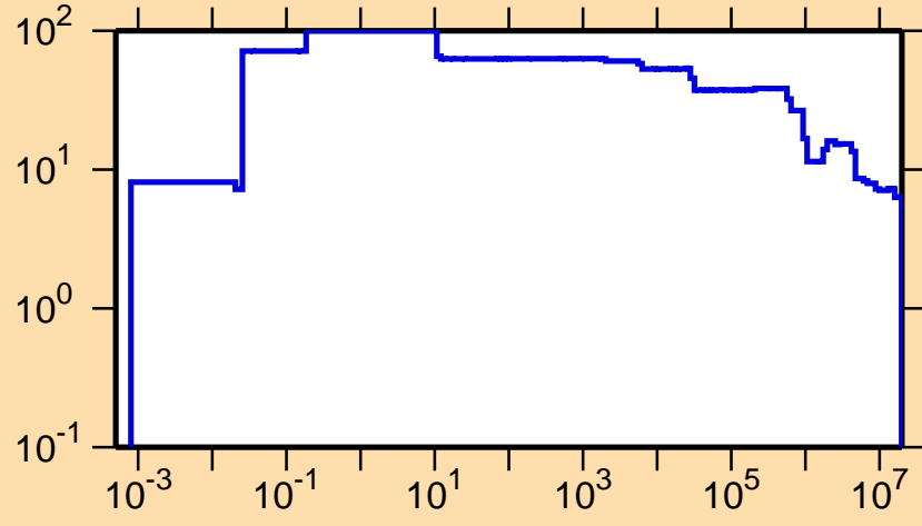
\Delta\sigma/\sigma vs. E for ^{163}\text{Lu}(n,\text{nonel.})
