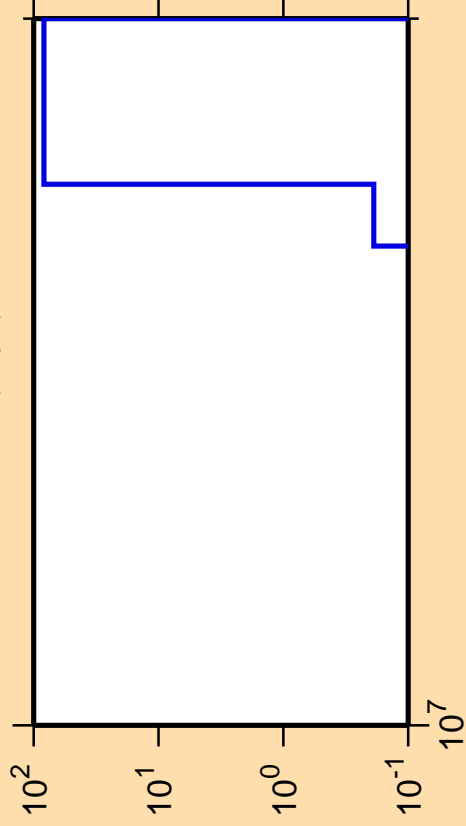
\Delta\sigma/\sigma vs. E for ^{163}\text{Lu}(n,\text{pt})
