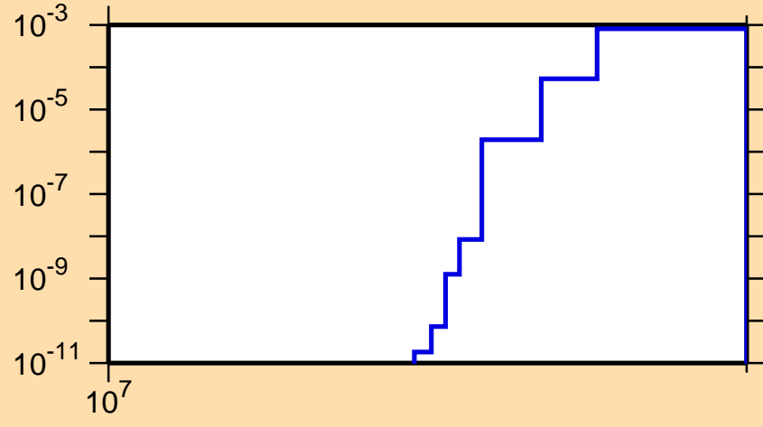
\sigma vs. E for ^{163}\text{Lu}(n,2np)
