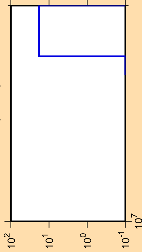
\Delta\sigma/\sigma vs. E for ^{163}\text{Lu} (mt 34)
