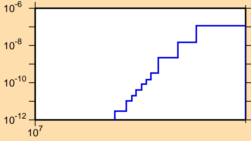
\sigma vs. E for ^{163}\text{Lu}(n,pd)
