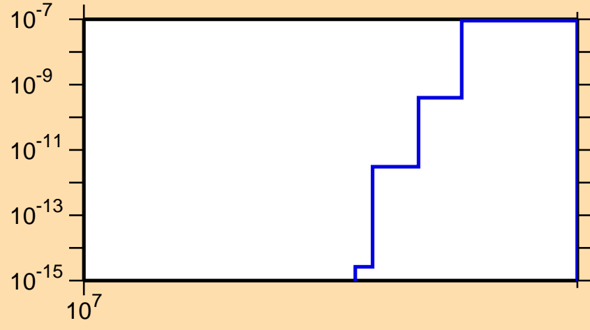
\sigma vs. E for ^{163}\text{Lu}(n,nt)
