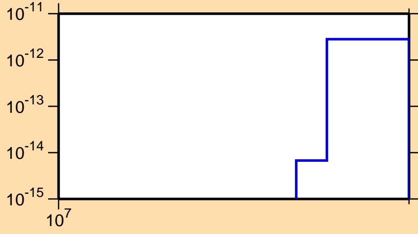
\sigma vs. E for ^{163}\text{Lu} (mt 34)
