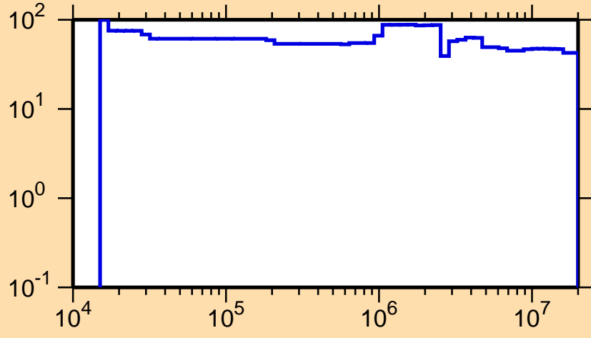
\Delta\sigma/\sigma vs. E for ^{163}\text{Lu}(n,n_1)
