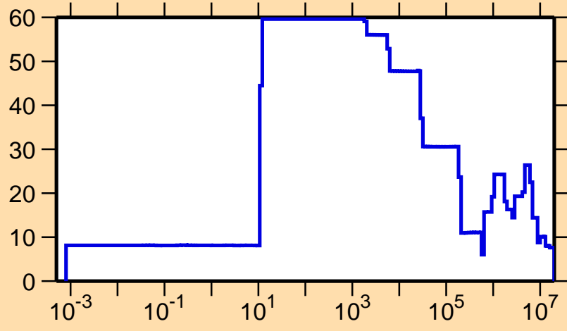
\Delta\sigma/\sigma vs. E for ^{163}\text{Lu}(n,\text{el.})
