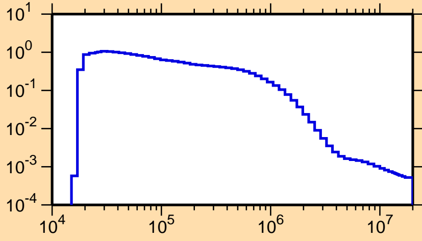
\sigma vs. E for ^{163}\text{Lu}(n,n_1)
