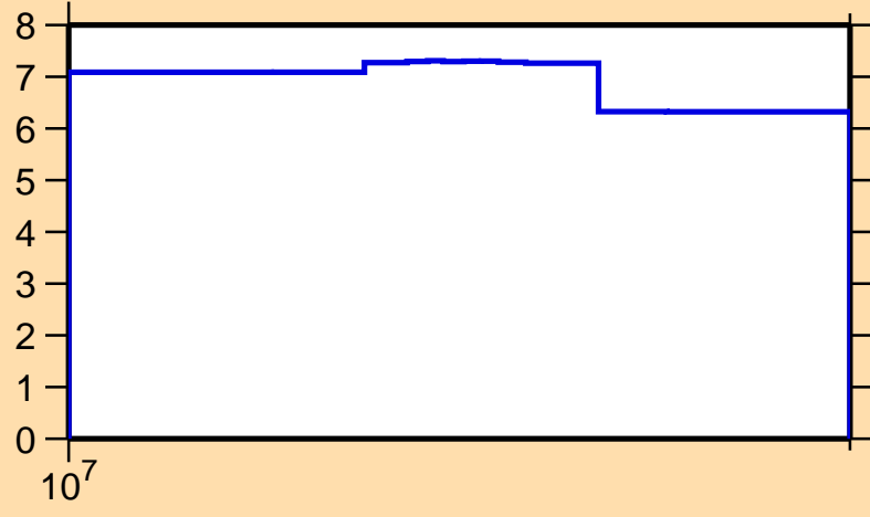
\Delta\sigma/\sigma vs. E for ^{163}\text{Lu}(n,\text{nonel.})
