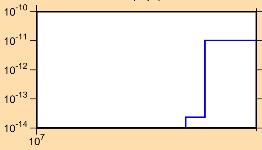
\sigma vs. E for ^{163}\text{Lu}(n,\text{pt})
