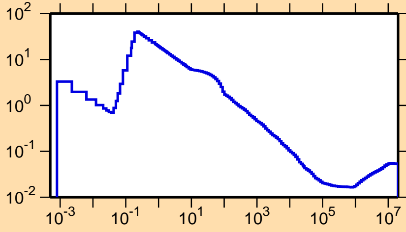
\sigma vs. E for ^{163}\text{Lu}(n,p)
