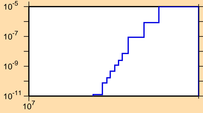
\sigma vs. E for ^{163}\text{Lu}(n,2n\alpha)
