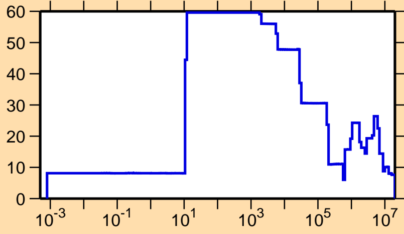
\Delta\sigma/\sigma vs. E for ^{163}\text{Lu}(n,\text{el.})
