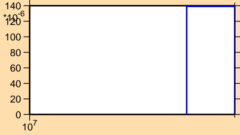
\sigma vs. E for ^{163}\text{Lu}(n,3n)
