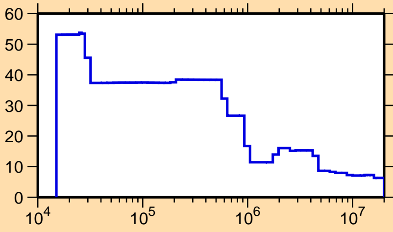
\Delta\sigma/\sigma vs. E for ^{163}\text{Lu}(n,\text{nonel.})
