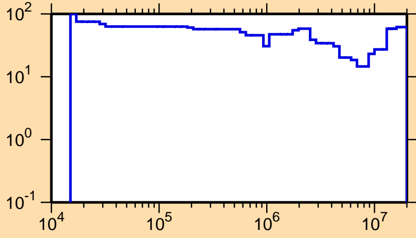
\Delta\sigma/\sigma vs. E for ^{163}\text{Lu}(n,\text{inel.})
