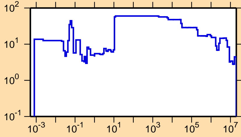
\Delta\sigma/\sigma vs. E for ^{163}\text{Lu}(n,\text{tot.})
