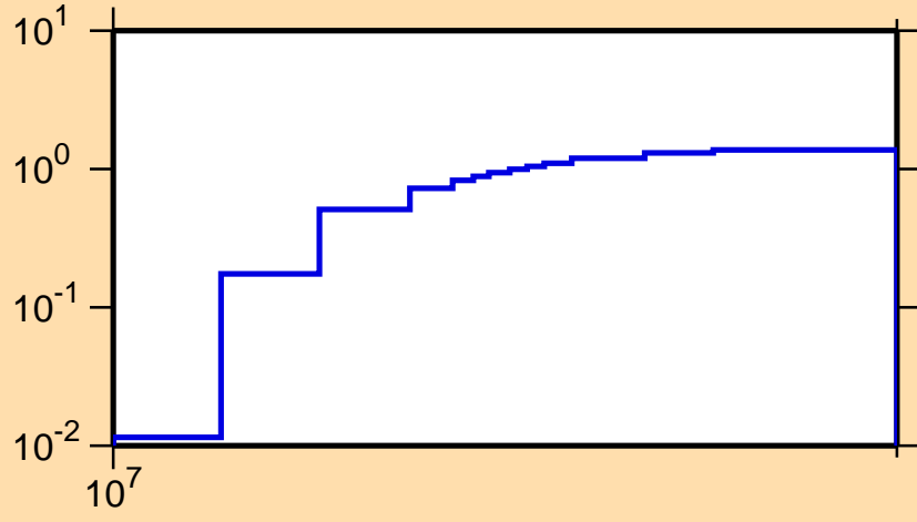
\sigma vs. E for ^{163}\text{Lu}(n,2n)
