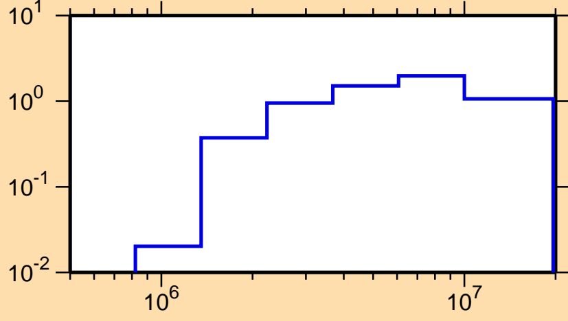
\sigma vs. E for ^{163}\text{Lu}(n,n\text{cont.})
