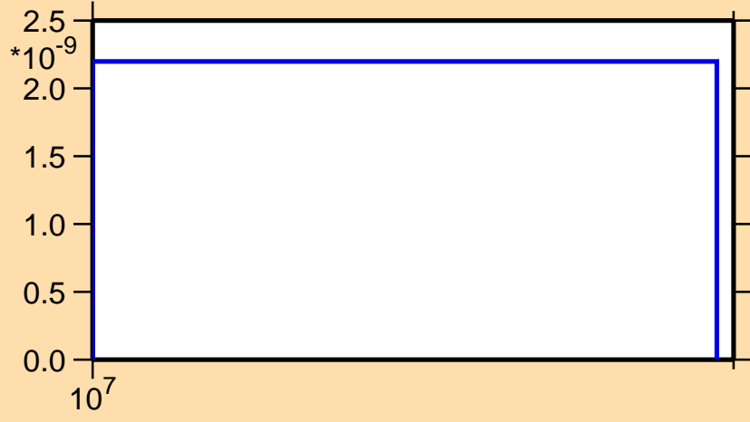
\sigma vs. E for ^{163}\text{Lu}(n,\text{pd})
