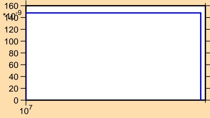
\sigma vs. E for ^{163}\text{Lu}(n,2n\alpha)
