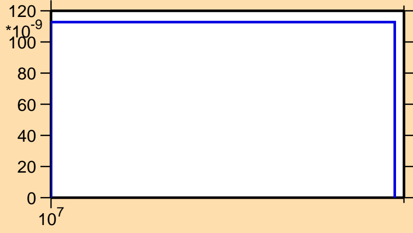
\sigma vs. E for ^{163}\text{Lu}(n,\text{nd})
