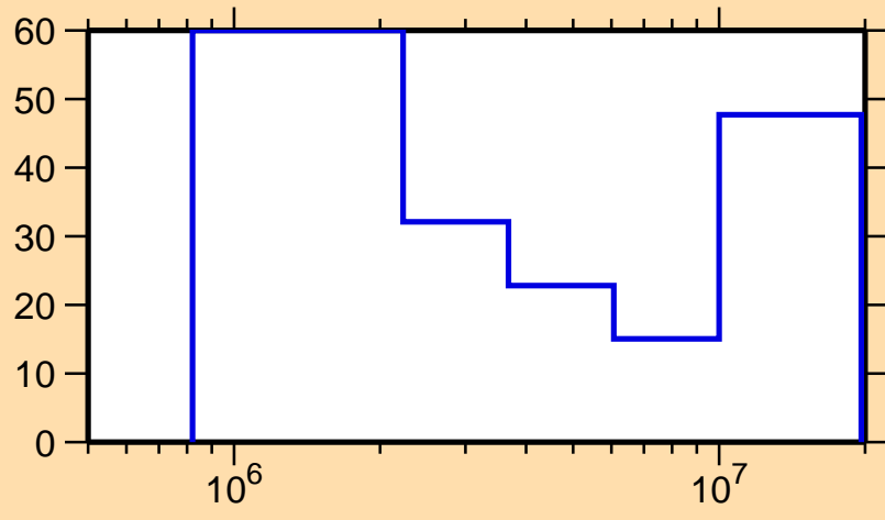
\Delta\sigma/\sigma vs. E for ^{163}\text{Lu}(n,n\text{cont.})
