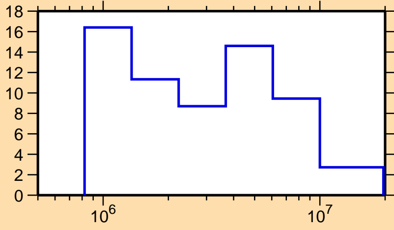
\Delta\sigma/\sigma vs. E for ^{163}\text{Lu}(n,\text{tot.})
