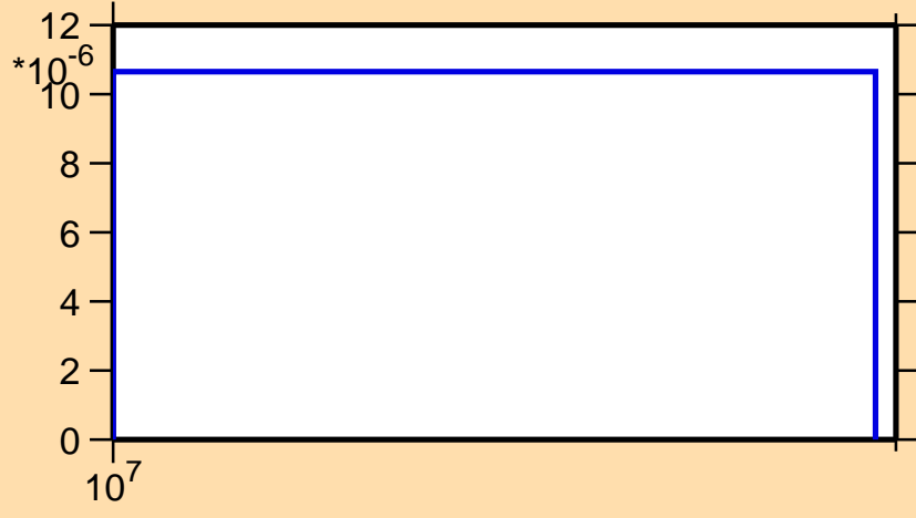
\sigma vs. E for ^{163}\text{Lu}(n,2np)
