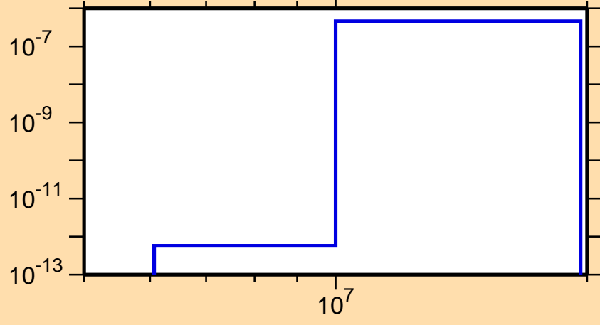
\sigma vs. E for ^{163}\text{Lu}(n,\text{He3})
