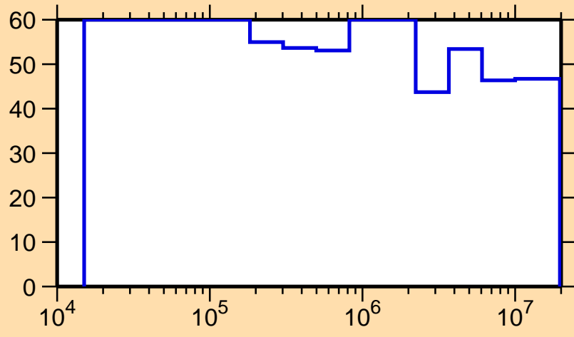
\Delta\sigma/\sigma vs. E for ^{163}\text{Lu}(n,n_1)
