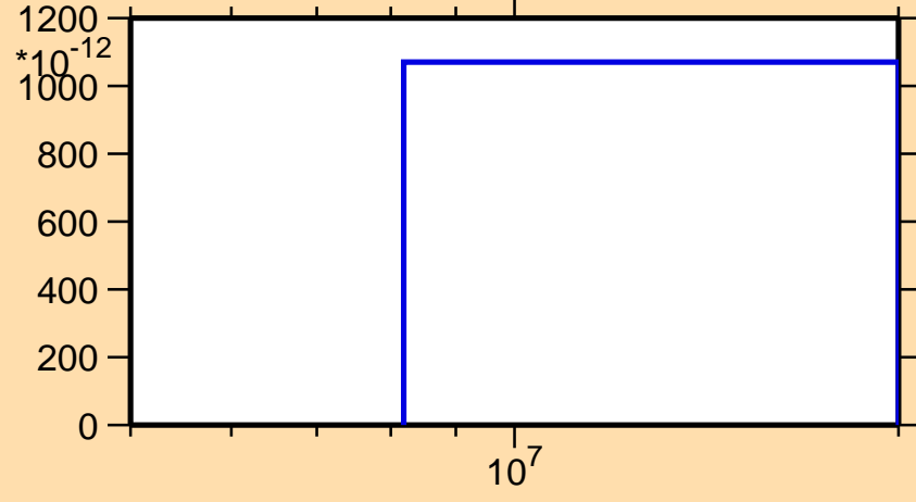
\sigma vs. E for ^{163}\text{Lu}(\text{mt117})
