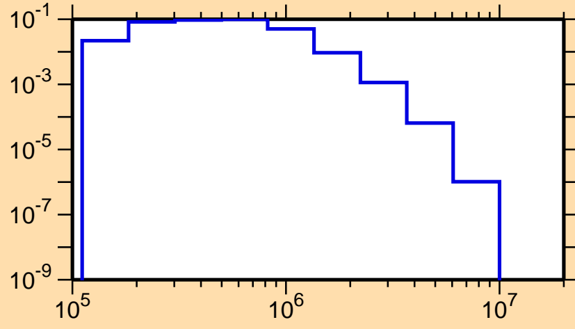
\sigma vs. E for ^{164}\text{Lu}(n,n_2)
