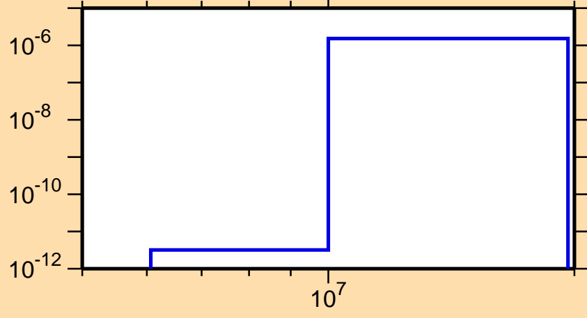
\sigma vs. E for ^{164}\text{Lu}(n,\text{He3})
