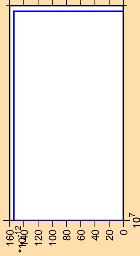
\Delta\sigma/\sigma vs. E for ^{164}\text{Lu} (mt 11)
