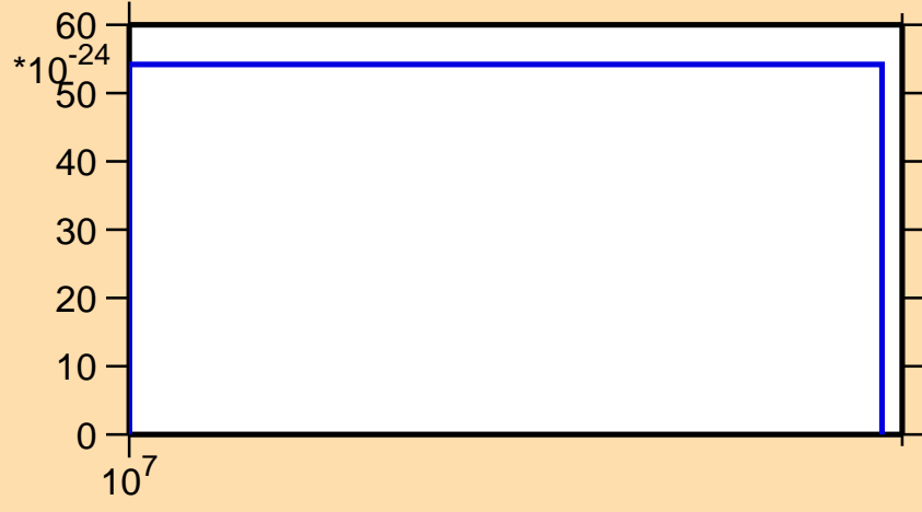
\sigma vs. E for ^{164}\text{Lu} (mt 11)
