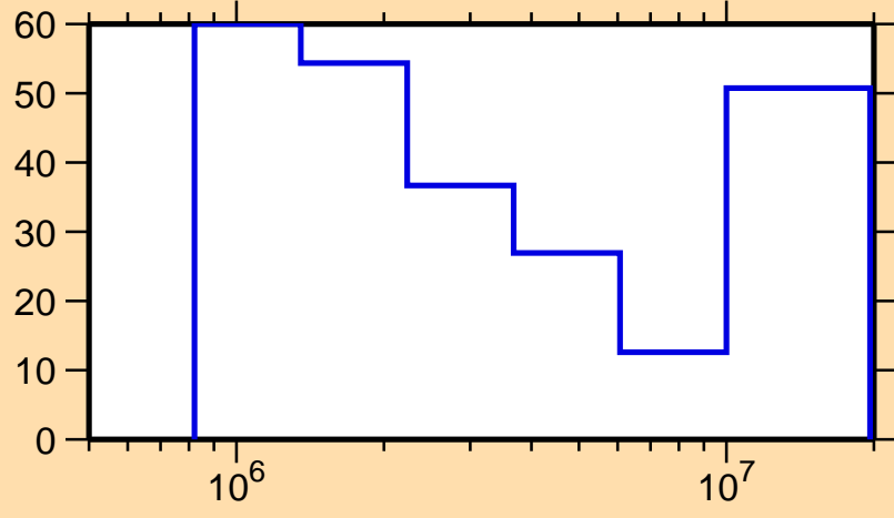
\Delta\sigma/\sigma vs. E for ^{164}\text{Lu}(n,n\text{cont.})
