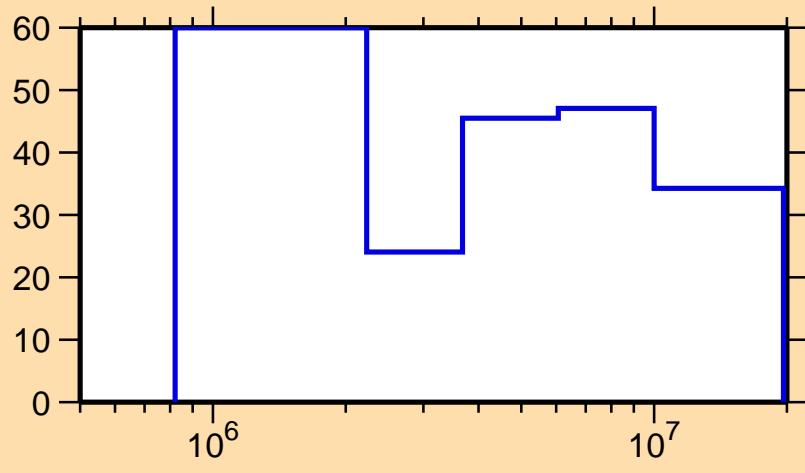
\Delta\sigma/\sigma vs. E for ^{164}\text{Lu}(n,n_1)
