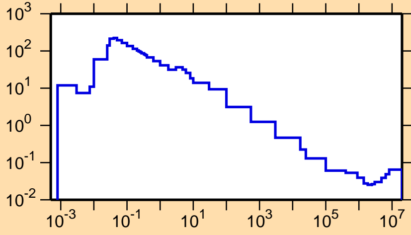
\sigma vs. E for ^{164}\text{Lu}(n,p)
