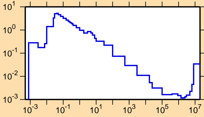
\sigma vs. E for ^{164}\text{Lu}(n,\alpha)
