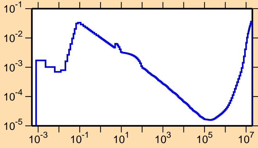
\sigma vs. E for ^{165}\text{Lu}(n,\alpha)
