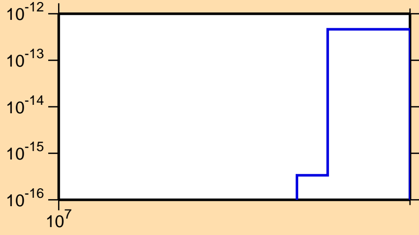
\sigma vs. E for ^{165}\text{Lu} (mt 34)
