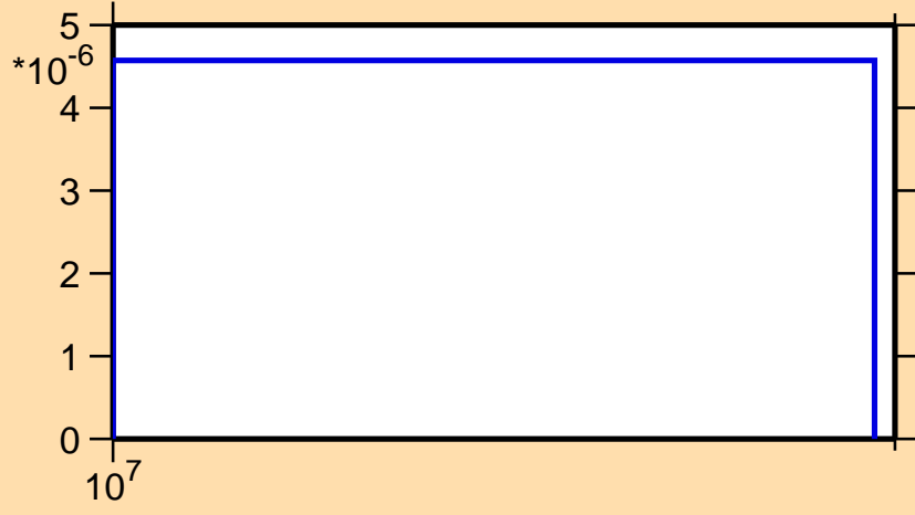
\sigma vs. E for ^{165}\text{Lu}(n,2np)
