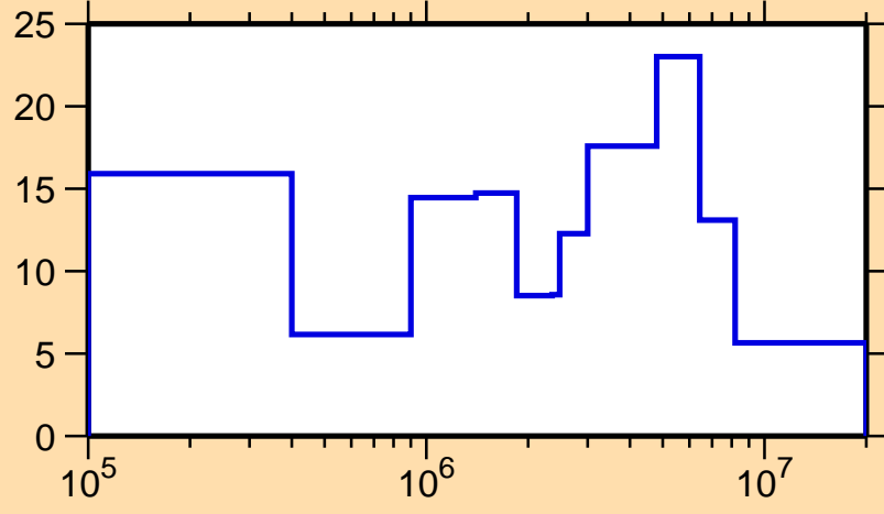
\Delta\sigma/\sigma vs. E for ^{165}\text{Lu}(n, el.)
