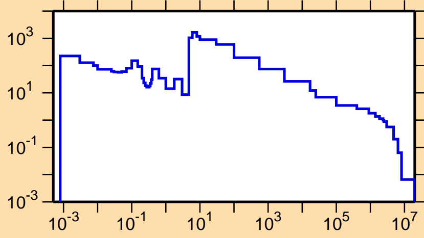
\sigma vs. E for ^{165}\text{Lu}(n,\gamma)
