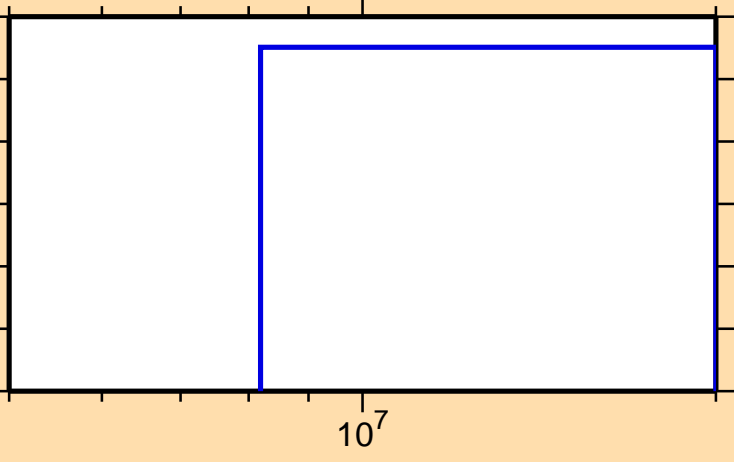
\sigma vs. E for ^{165}\text{Lu} (mt 45)
