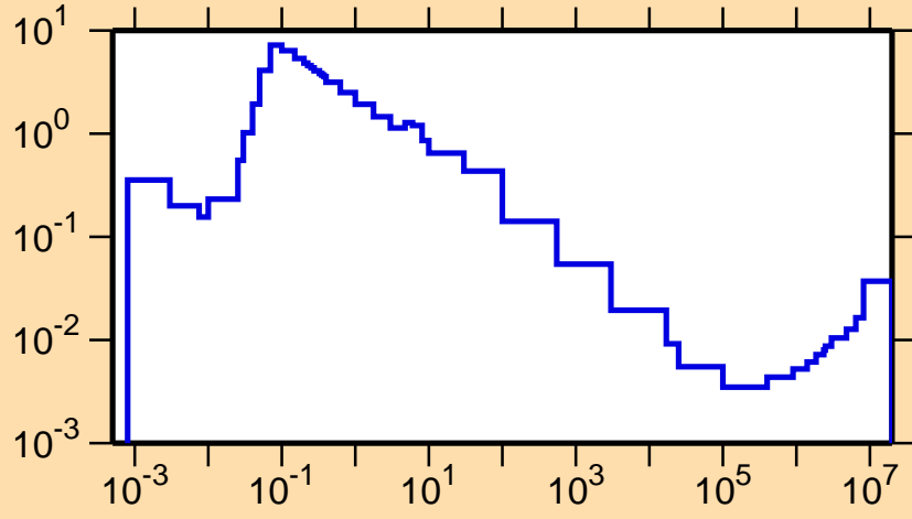
\sigma vs. E for ^{165}\text{Lu}(n,p)
