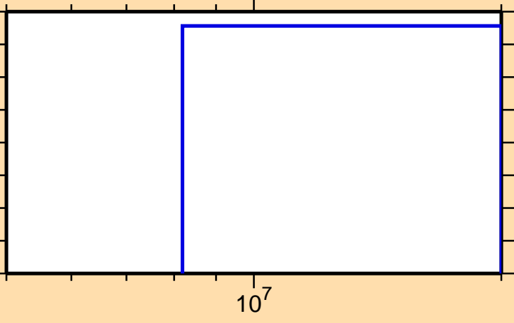
\sigma vs. E for ^{165}\text{Lu}(n,nt)
