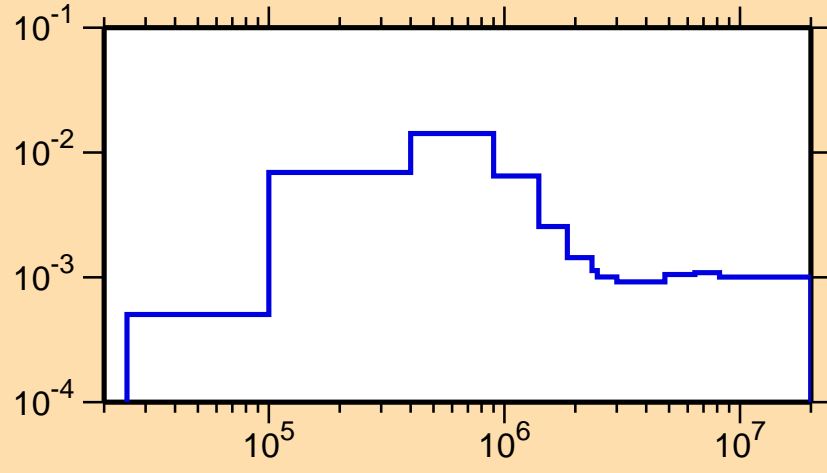
\sigma vs. E for ^{166}\text{Lu}(n,n_1)
