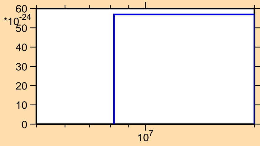
\sigma vs. E for ^{166}\text{Lu}(\text{mt } 11)
