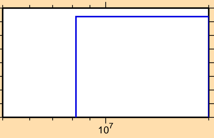
\sigma vs. E for ^{166}\text{Lu}(n,\text{nd})
