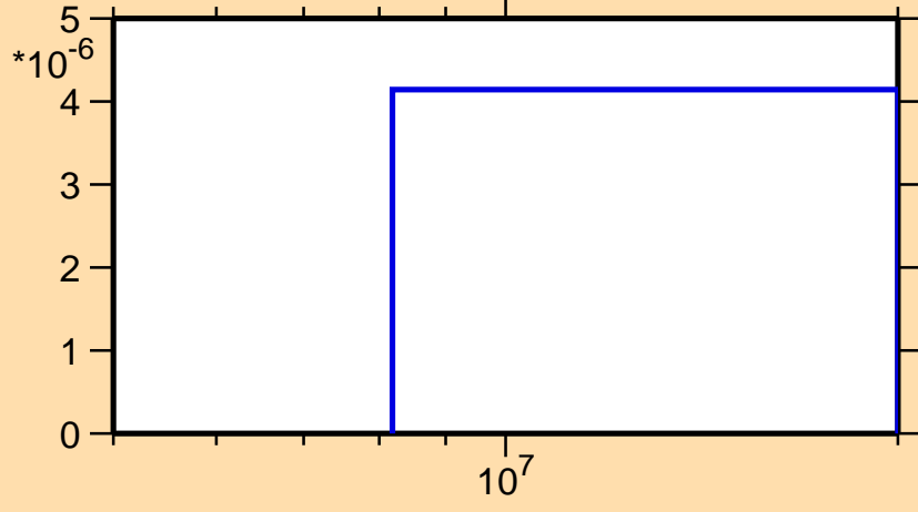
\sigma vs. E for ^{166}\text{Lu}(n,3n)
