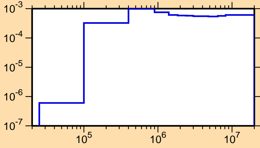
\sigma vs. E for ^{166}\text{Lu}(n,n_3)
