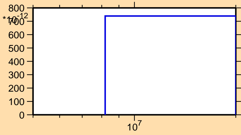
\sigma vs. E for ^{166}\text{Lu}(\text{mt } 45)
