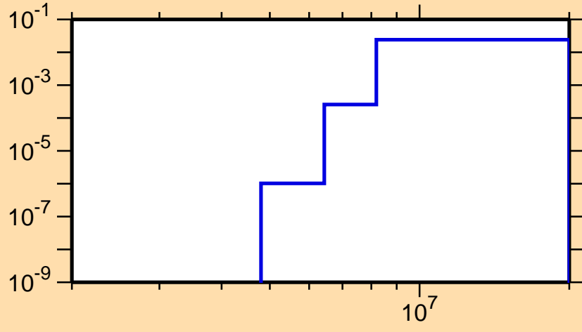
\sigma vs. E for ^{166}\text{Lu}(n,np)
