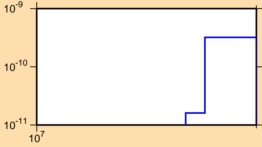
\sigma vs. E for ^{167}\text{Lu}(n,\text{pd})
