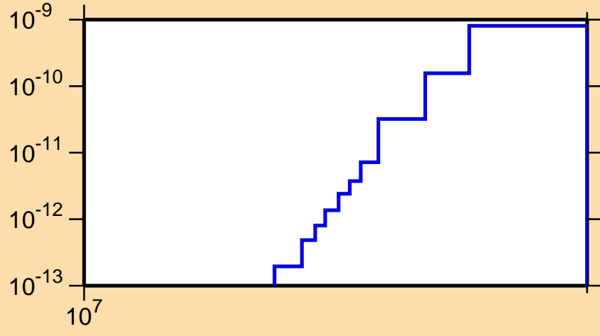
\sigma vs. E for ^{167}\text{Lu}(\text{mt117})
