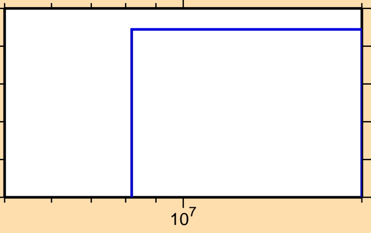
\sigma vs. E for ^{167}\text{Lu}(n,2n\alpha)
