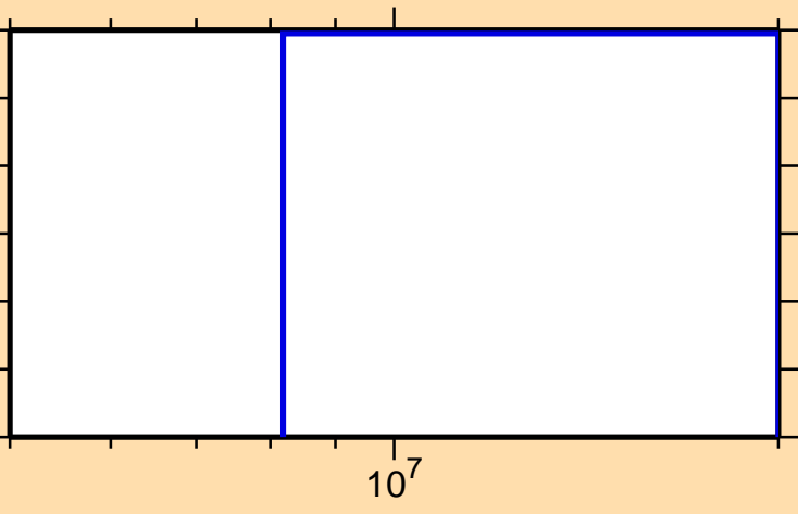
\sigma vs. E for ^{167}\text{Lu} (mt 34)
