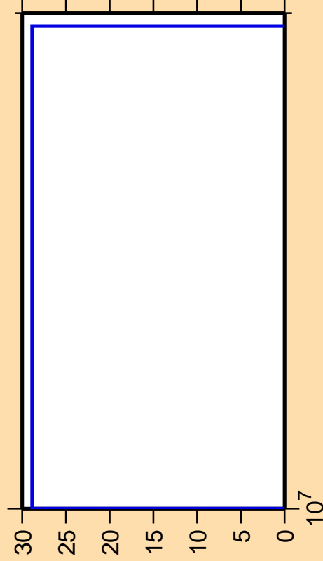
\Delta\sigma/\sigma vs. E for ^{167}\text{Lu}(n,pd)
