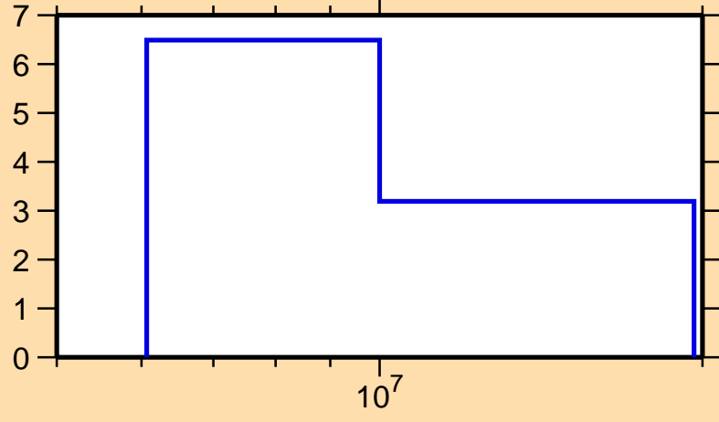
\Delta\sigma/\sigma vs. E for ^{167}\text{Lu}(n,\text{tot.})
