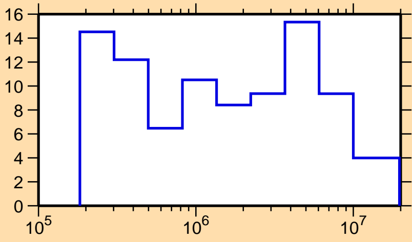
\Delta\sigma/\sigma vs. E for ^{167}\text{Lu}(n, el.)
