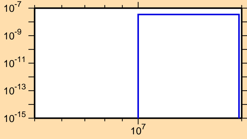
\sigma vs. E for ^{167}\text{Lu}(n,\text{He3})
