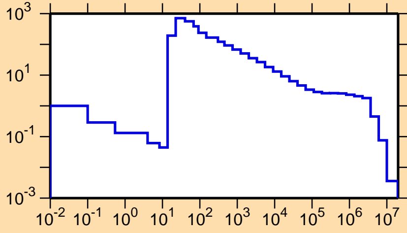
\sigma vs. E for ^{167}\text{Lu}(n,\gamma)
