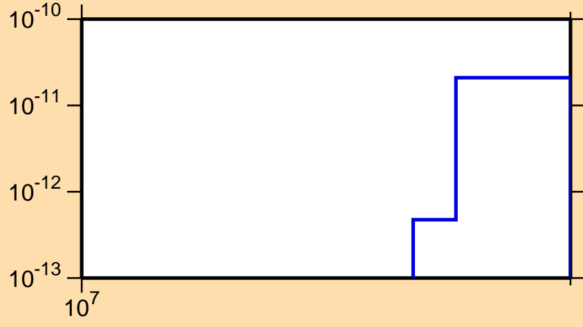
\sigma vs. E for ^{168}\text{Lu}(n,\text{pd})
