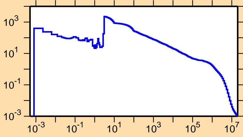
\sigma vs. E for ^{168}\text{Lu}(n,\gamma)
