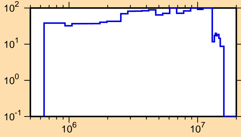
\Delta\sigma/\sigma vs. E for ^{168}\text{Lu}(n,n_1)
