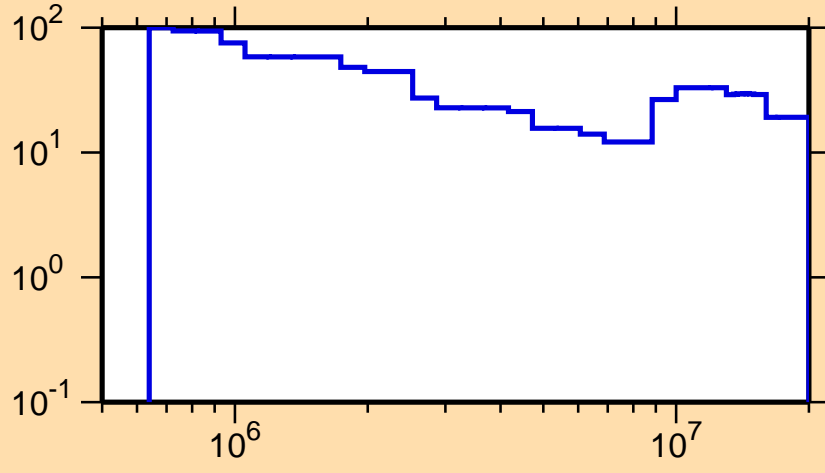
\Delta\sigma/\sigma vs. E for ^{168}\text{Lu}(n,n\text{cont.})
