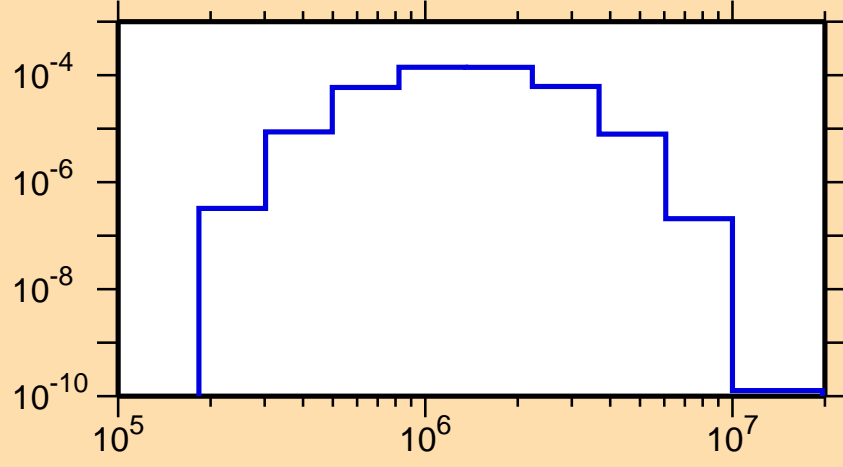
\sigma vs. E for ^{168}\text{Lu}(n,n_2)
