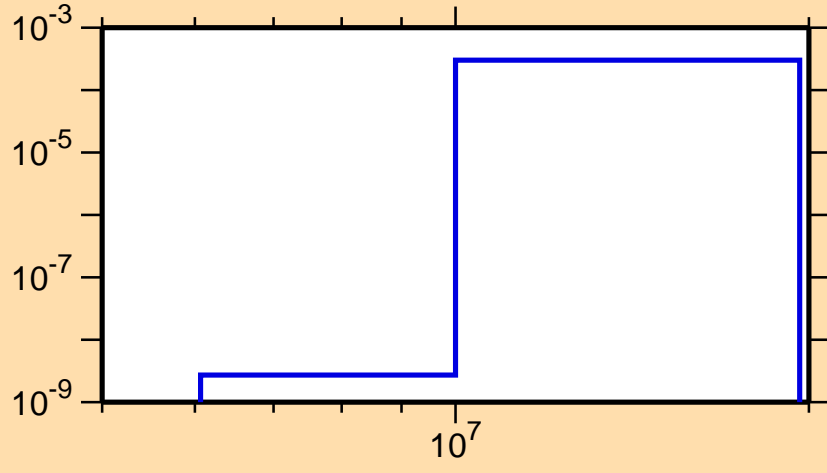
\sigma vs. E for ^{168}\text{Lu}(n,t)
