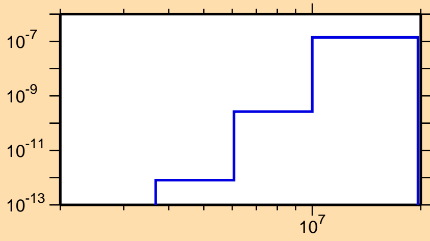
\sigma vs. E for ^{168}\text{Lu}(n,p\alpha)
