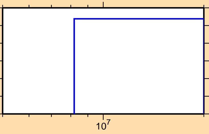
\sigma vs. E for ^{168}\text{Lu}(n,\text{pt})
