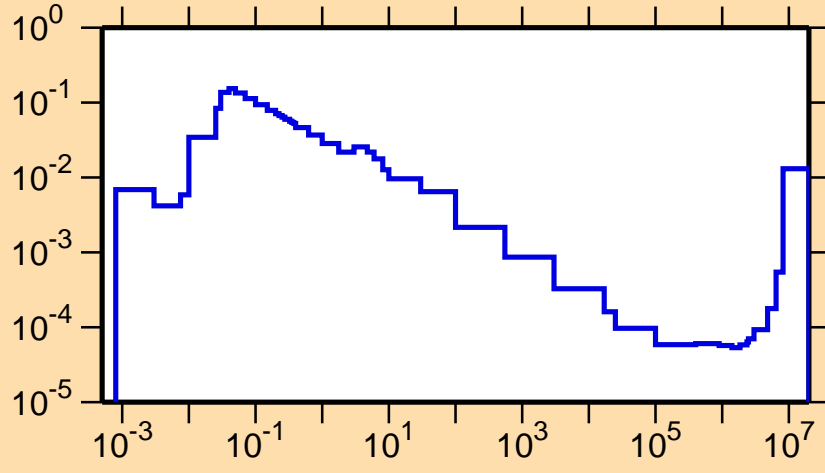
\sigma vs. E for ^{168}\text{Lu}(n,\alpha)
