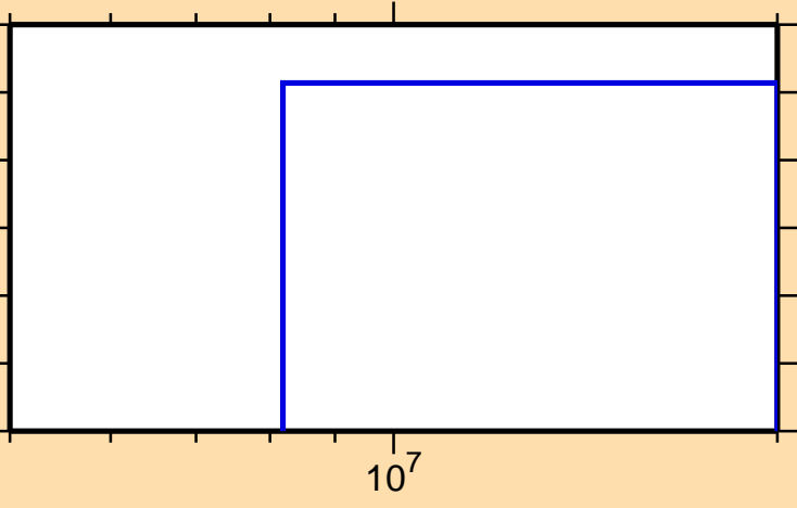
\sigma vs. E for ^{168}\text{Lu}(n,\text{He3})
