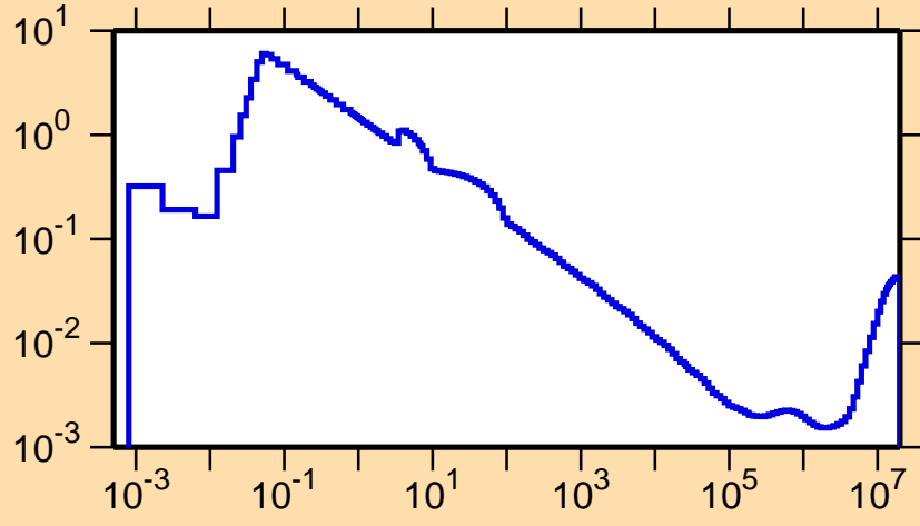
\sigma vs. E for ^{168}\text{Lu}(n,p)
