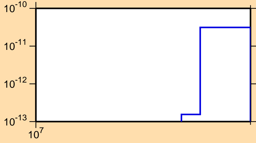
\sigma vs. E for ^{168}\text{Lu} (mt 34)
