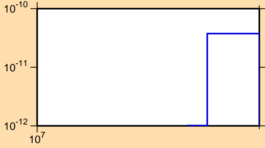
\sigma vs. E for ^{168}\text{Lu}(n,pd)
