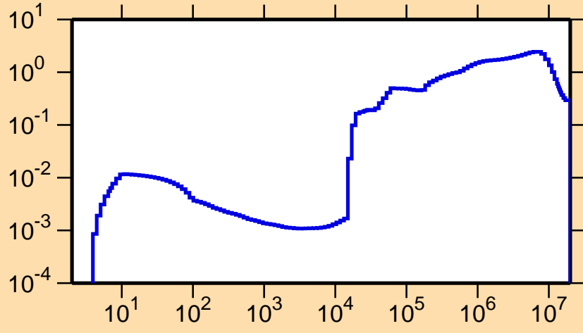
\sigma vs. E for ^{168}\text{Lu}(n,\text{inel.})
