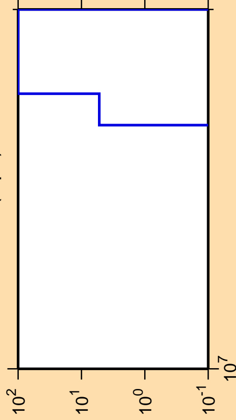
\Delta\sigma/\sigma vs. E for ^{168}\text{Lu}(n,pd)
