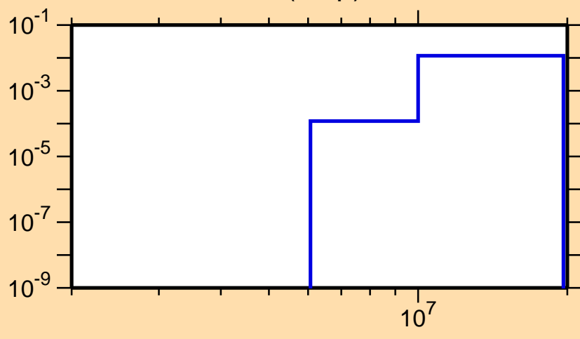
\sigma vs. E for ^{168}\text{Lu}(n,np)
