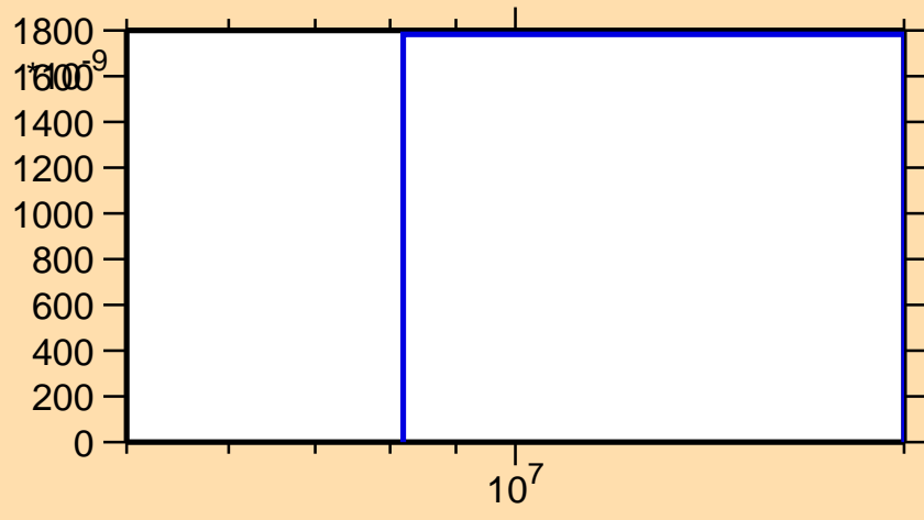
\sigma vs. E for ^{168}\text{Lu}(n,nd)
