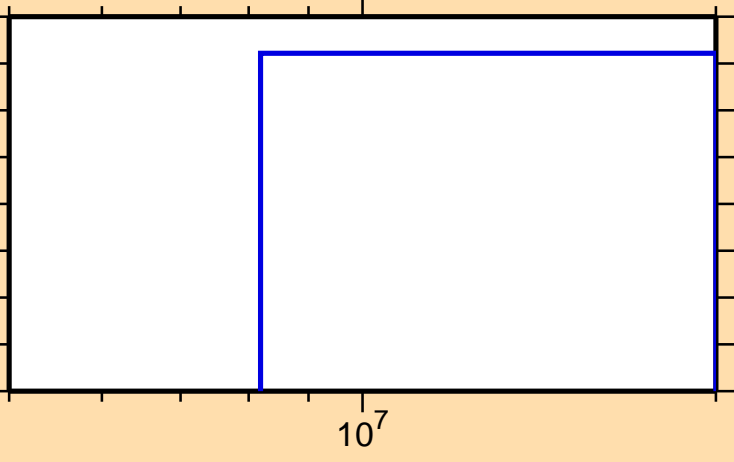
\sigma vs. E for ^{168}\text{Lu}(n,3n)
