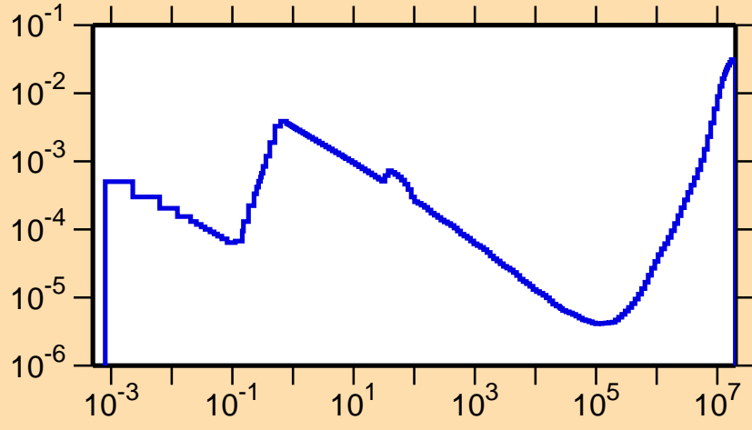
\sigma vs. E for ^{169}\text{Lu}(n,p)
