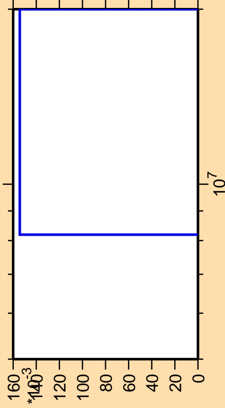
\Delta\sigma/\sigma vs. E for ^{169}\text{Lu}(n,pd)
