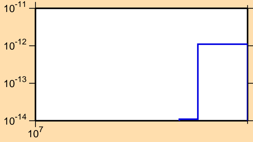
\sigma vs. E for ^{170}\text{Lu}(n,pd)
