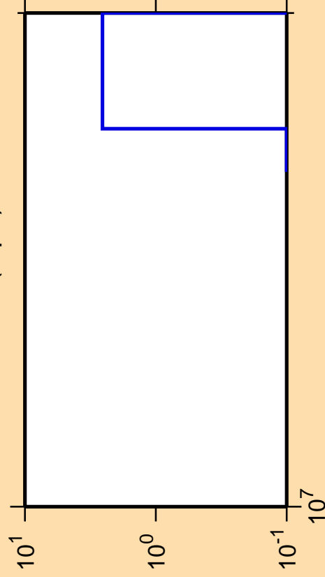
\Delta\sigma/\sigma vs. E for ^{170}\text{Lu}(n,pd)
