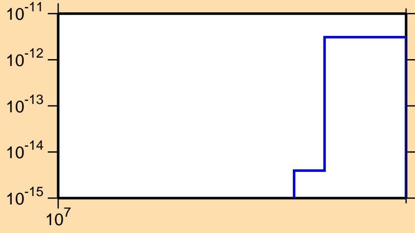
\sigma vs. E for ^{170}\text{Lu} (mt 34)
