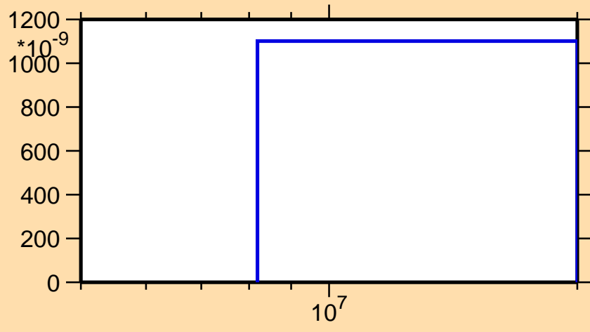
\sigma vs. E for ^{170}\text{Lu}(n,\text{nd})
