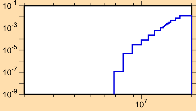
\sigma vs. E for ^{171}\text{Lu}(n,np)
