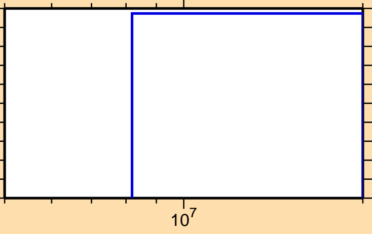
\sigma vs. E for ^{171}\text{Lu}(n,3n)
