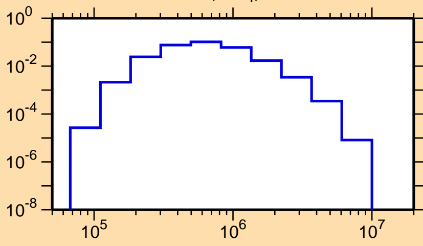
\sigma vs. E for ^{171}\text{Lu}(n,n_4)
