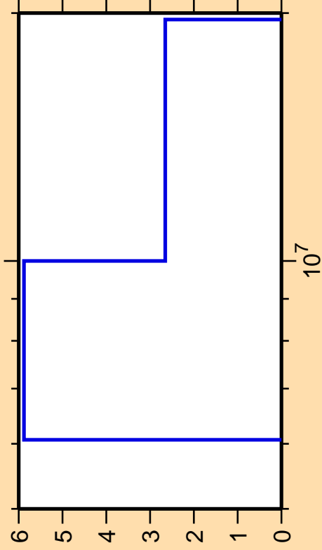
\Delta\sigma/\sigma vs. E for ^{171}\text{Lu}(n,2n)
