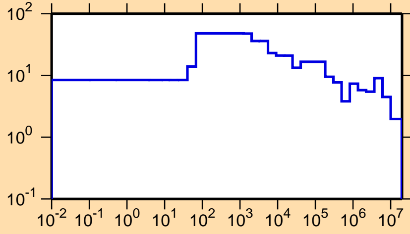
\Delta\sigma/\sigma vs. E for ^{171}\text{Lu}(n,el.)
