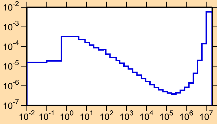
\sigma vs. E for ^{171}\text{Lu}(n,\alpha)
