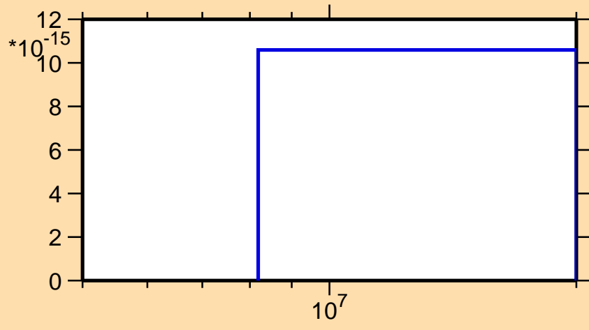
\sigma vs. E for ^{172}\text{Lu} (mt 45)
