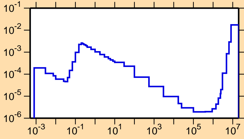
\sigma vs. E for ^{172}\text{Lu}(n,p)
