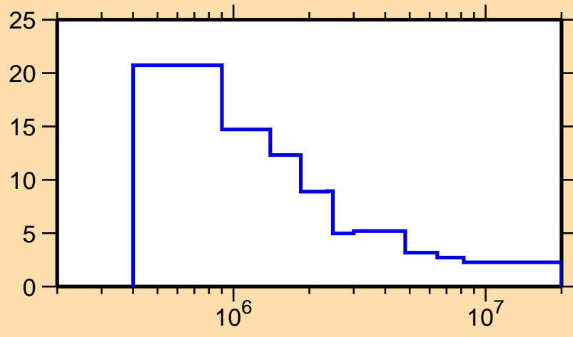
\Delta\sigma/\sigma vs. E for ^{172}\text{Lu}(n,n\text{onel.})
