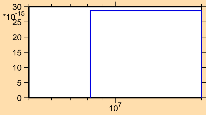
\sigma vs. E for ^{172}\text{Lu}(\text{mt117})
