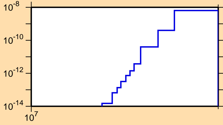
\sigma vs. E for ^{173}\text{Lu}(n,\text{He3})
