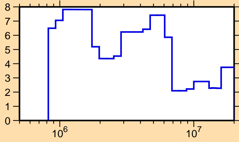
\Delta\sigma/\sigma vs. E for ^{173}\text{Lu}(n,\text{el.})
