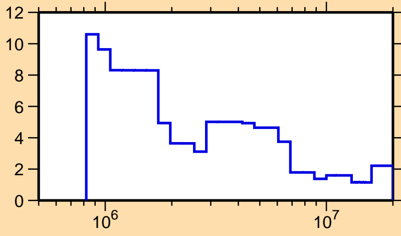
\Delta\sigma/\sigma vs. E for ^{173}\text{Lu}(n,\text{tot.})
