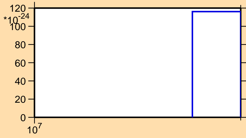
\sigma vs. E for ^{173}\text{Lu} (mt 42)
