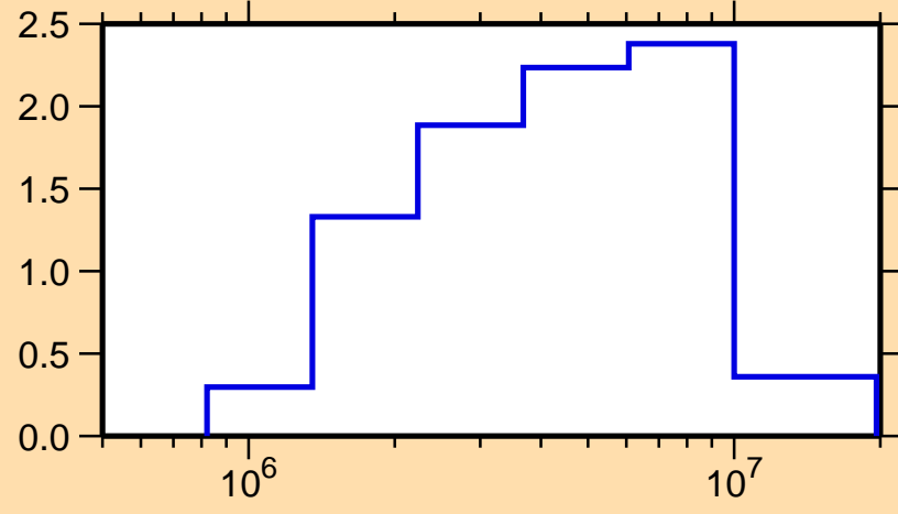
\sigma vs. E for ^{173}\text{Lu}(n,n\text{cont.})
