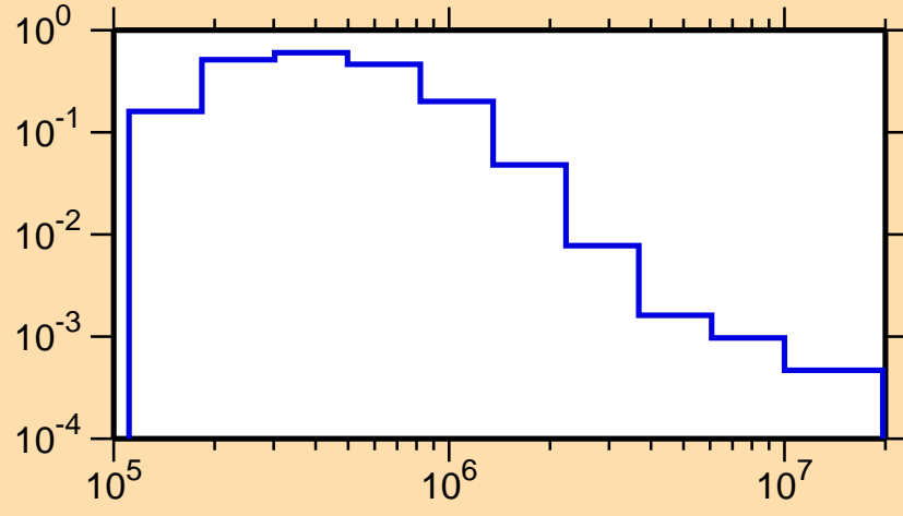
\sigma vs. E for ^{173}\text{Lu}(n,n_1)
