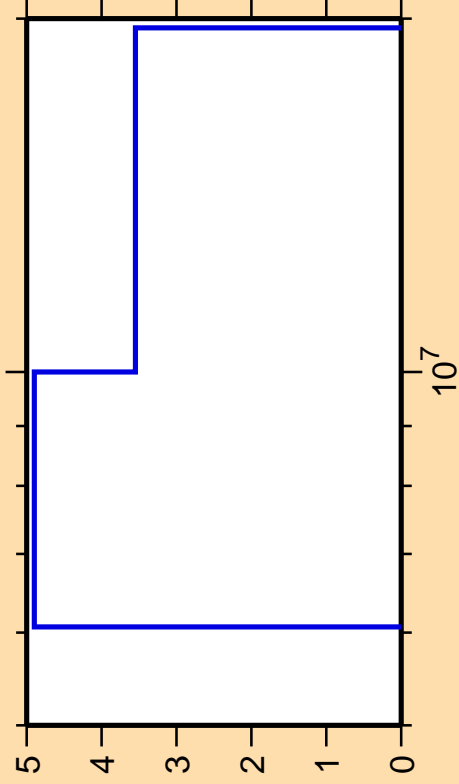
\Delta\sigma/\sigma vs. E for ^{173}\text{Lu}(n,2n)
