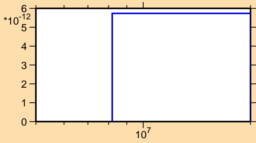
\sigma vs. E for ^{173}\text{Lu}(n,p\alpha)
