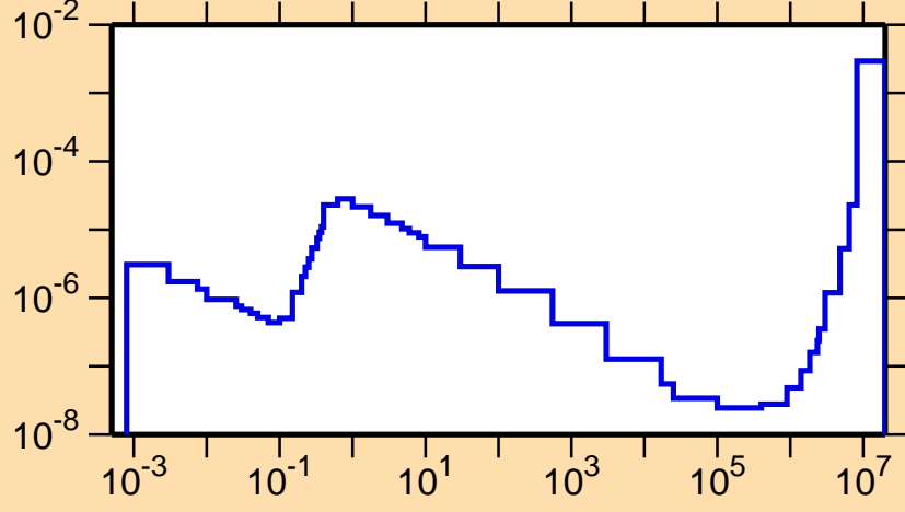
\sigma vs. E for ^{173}\text{Lu}(n,\alpha)
