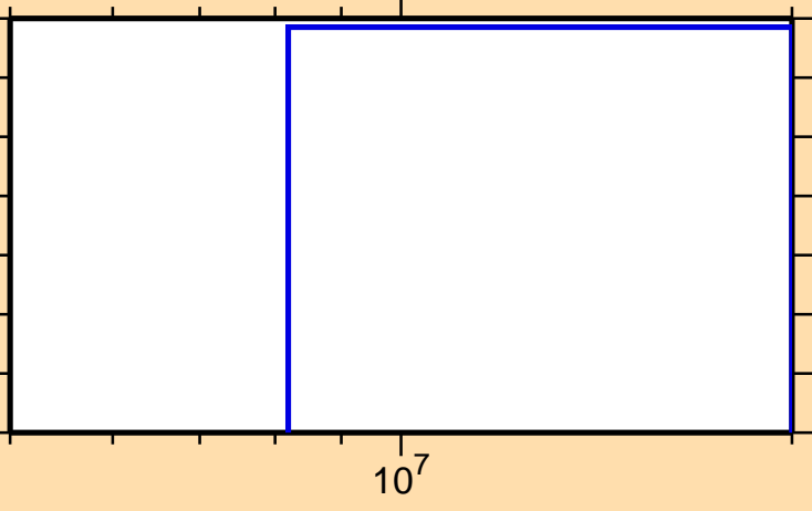
\sigma vs. E for ^{173}\text{Lu}(n,nt)
