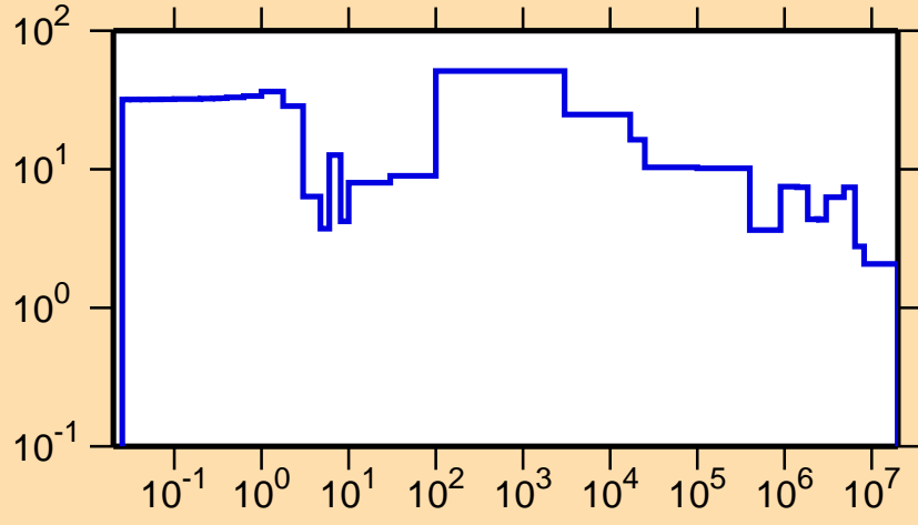
\Delta\sigma/\sigma vs. E for ^{173}\text{Lu}(n,el.)
