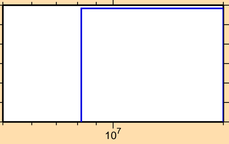
\sigma vs. E for ^{173}\text{Lu}(n,t)
