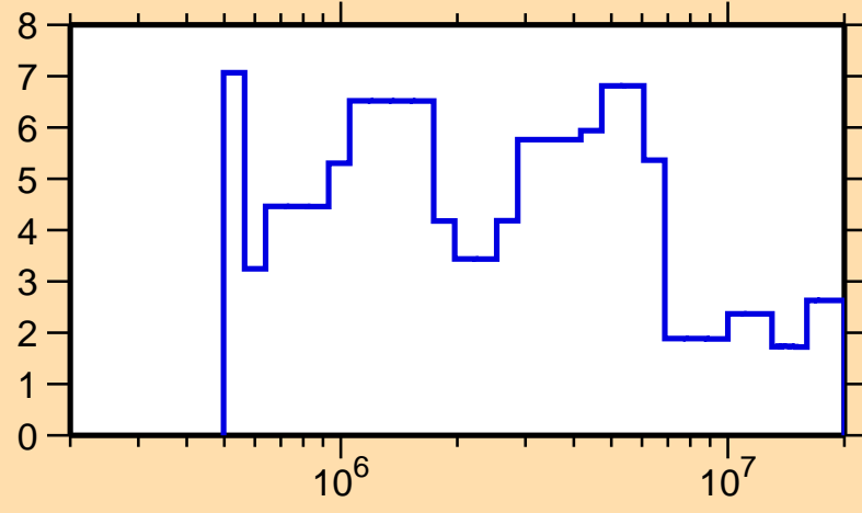
\Delta\sigma/\sigma vs. E for ^{174}\text{Lu}(n, el.)
