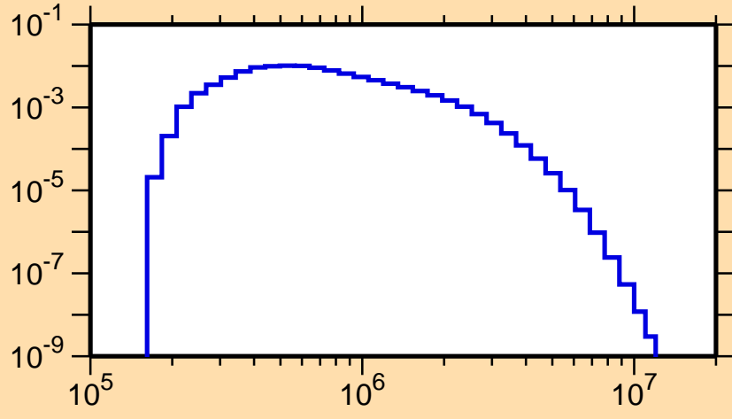
\sigma vs. E for ^{174}\text{Lu}(n,n_3)
