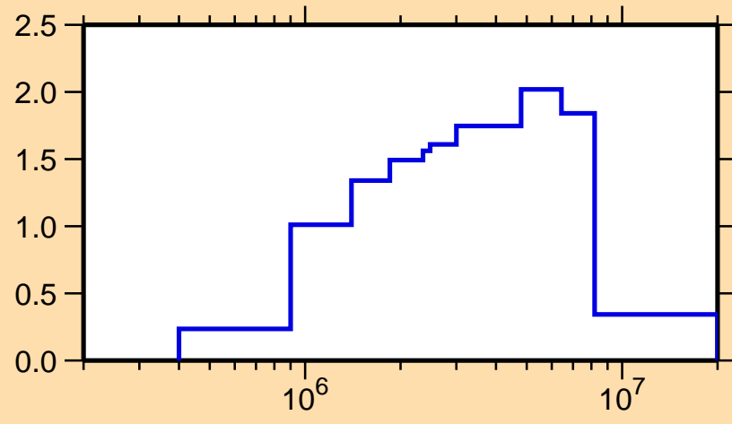
\sigma vs. E for ^{174}\text{Lu}(n,n\text{cont.})
