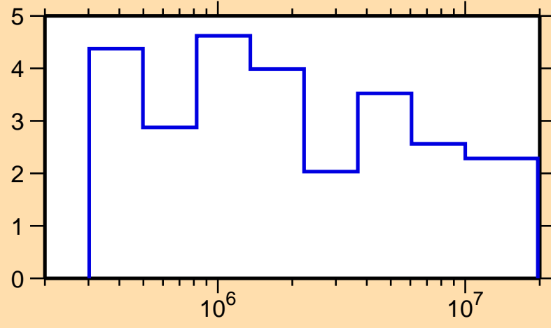
\Delta\sigma/\sigma vs. E for ^{174}\text{Lu}(n,\text{el.})
