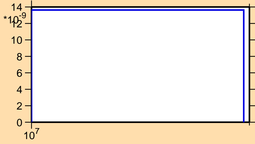
\sigma vs. E for ^{174}\text{Lu}(n,nt)
