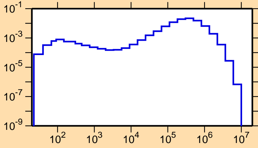
\sigma vs. E for ^{174}\text{Lu}(n,n_2)
