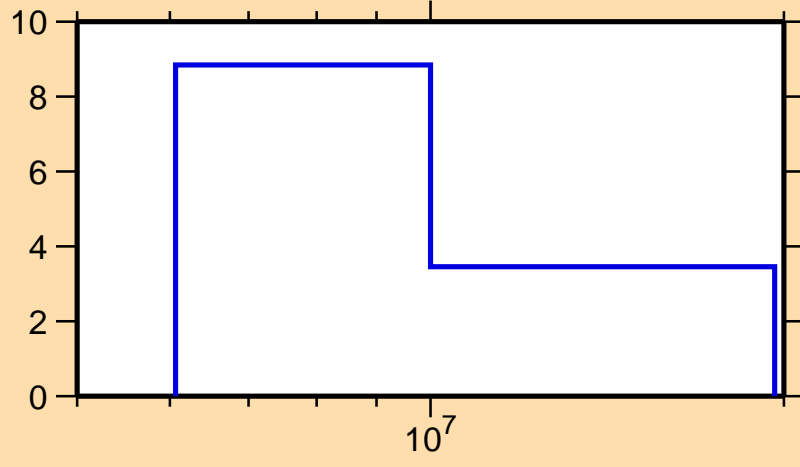
\Delta\sigma/\sigma vs. E for ^{174}\text{Lu}(n,2n)
