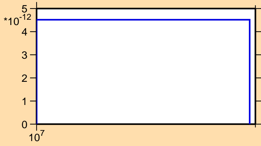
\sigma vs. E for ^{174}\text{Lu}(n,p\alpha)
